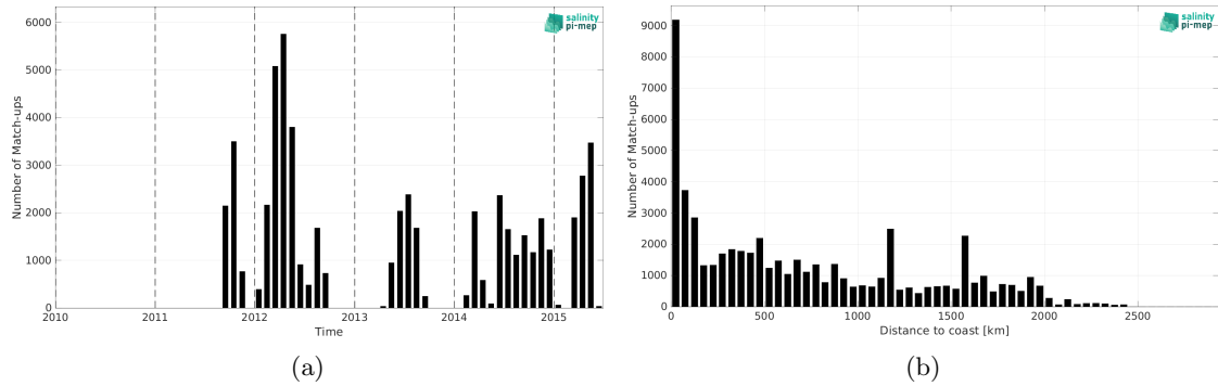
Figure 2: Number of match-ups between TSG (SAMOS) and Aquarius SSS L3 CAP v5 - Monthly (JPL) SSS as a function of time (a) and as function of the distance to coast (b) over the Tropical Pacific Ocean Pi-MEP region and for the full satellite product period.
