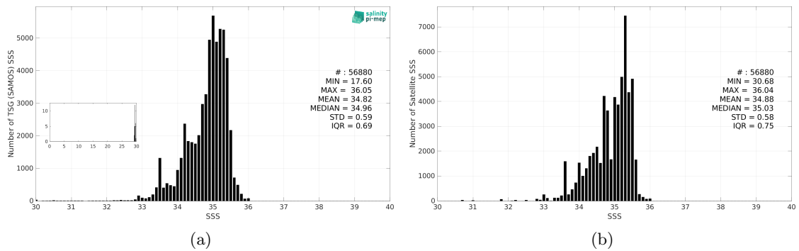
Figure 3: Histograms of SSS from TSG (SAMOS) (a) and Aquarius SSS L3 CAP v5 - Monthly (JPL) (b) considering all match-up pairs per bins of 0.1 over the Tropical Pacific Ocean Pi-MEP region and for the full satellite product period.
