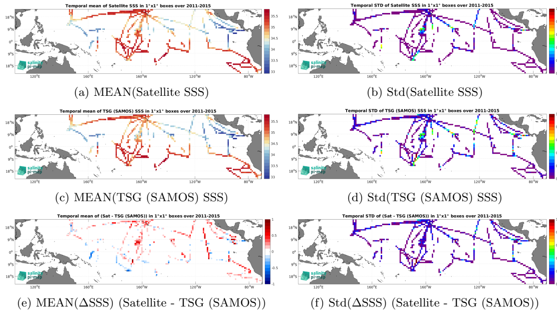
Figure 7: Temporal mean (left) and Std (right) of SSS from Aquarius SSS L3 CAP v5 - Monthly (JPL) (top), TSG (SAMOS) (middle), and of \Delta SSS (Satellite - TSG (SAMOS)). Only match-up pairs are used to generate these maps.
