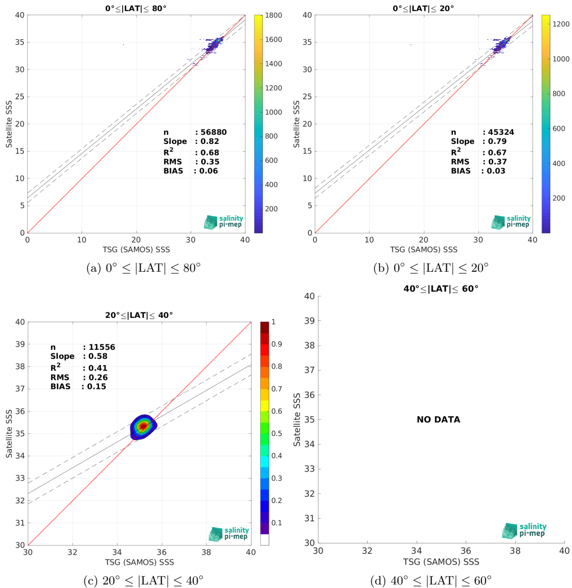
Figure 10: Contour maps of the concentration of Aquarius SSS L3 CAP v5 - Monthly (JPL) SSS (y-axis) versus TSG (SAMOS) SSS (x-axis) at match-up pairs for different latitude bands. For each plot, the red line shows x=y . The black thin and dashed lines indicate a linear fit through the data cloud and the \pm 95\% confidence levels, respectively. The number match-up pairs n , the slope and R^2 coefficient of the linear fit, the root mean square (RMS) and the mean bias between satellite and in situ data are indicated for each latitude band in each plot.
