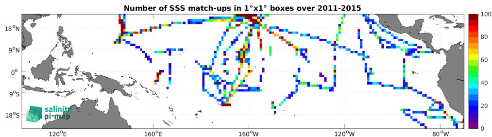
Figure 5: Number of SSS match-ups between TSG (SAMOS) SSS and the Aquarius SSS L3 CAP v5 - Monthly (JPL) SSS product for the Tropical Pacific Ocean Pi-MEP region over 1^\circ \times 1^\circ boxes and for the full satellite product period.
