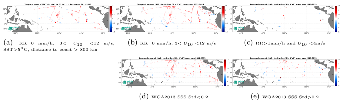
Figure 14: Temporal mean gridded over spatial boxes of size 1^\circ \times 1^\circ of \Delta SSS (Aquarius SSS L3 CAP v5 - Monthly (JPL) - TSG (SAMOS)) for 5 different subdatasets corresponding to: RR=0 mm/h, 3 < U_{10} < 12 m/s, SST > 5^\circ\text{C} , distance to coast > 800 km (a), RR=0 mm/h, 3 < U_{10} < 12 m/s (b), RR > 1 mm/h and U_{10} < 4 m/s (c), WOA2013 SSS Std < 0.2 (d), WOA2013 SSS Std > 0.2 (e).
