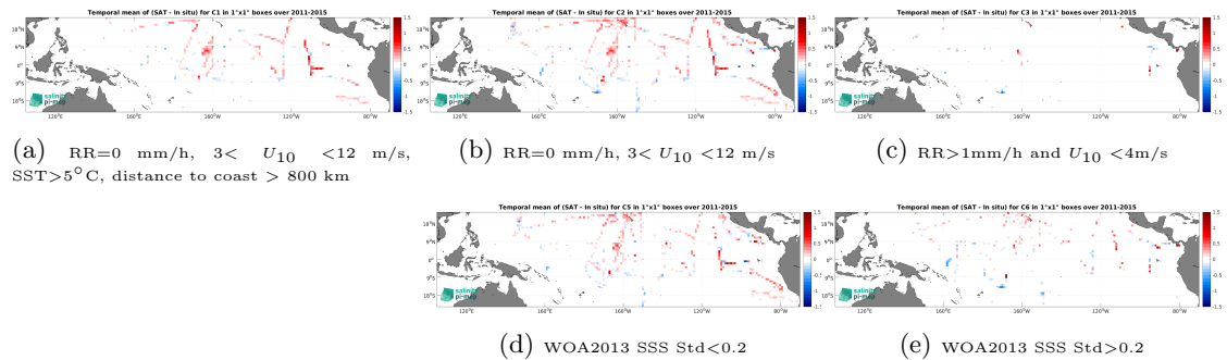
Figure 12: Temporal mean gridded over spatial boxes of size 1^\circ \times 1^\circ of \Delta SSS (Aquarius SSS L3 CAP v5 - Monthly (JPL) - TSG (SAMOS)) for 5 different subdatasets corresponding to: RR=0 mm/h, 3 < U_{10} < 12 m/s, SST > 5^\circ\text{C} , distance to coast > 800 km (a), RR=0 mm/h, 3 < U_{10} < 12 m/s (b), RR > 1 mm/h and U_{10} < 4 m/s (c), WOA2013 SSS Std < 0.2 (d), WOA2013 SSS Std > 0.2 (e).
