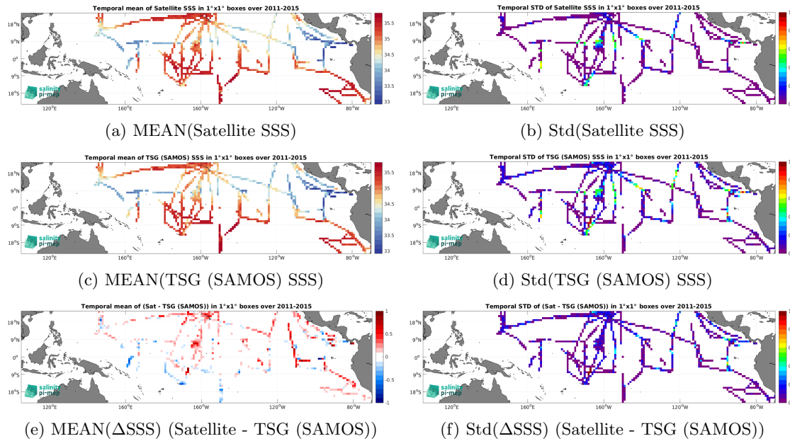
Figure 6: Temporal mean (left) and Std (right) of SSS from Aquarius SSS L3 CAP v5 - Monthly (JPL) (top), TSG (SAMOS) (middle), and of \Delta SSS (Satellite - TSG (SAMOS)). Only match-up pairs are used to generate these maps.
