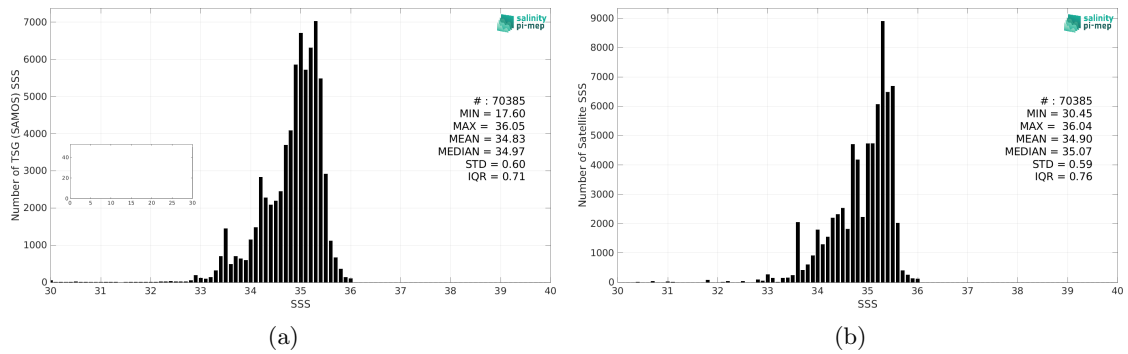
Figure 2: Histograms of SSS from TSG (SAMOS) (a) and Aquarius SSS L3 CAP v5 - Monthly (JPL) (b) considering all match-up pairs per bins of 0.1 over the Tropical Pacific Ocean Pi-MEP region and for the full satellite product period.
