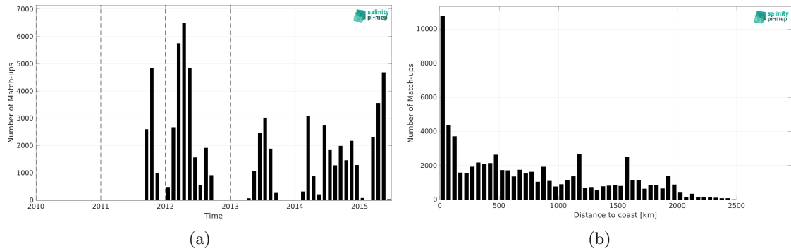
Figure 1: Number of match-ups between TSG (SAMOS) and Aquarius SSS L3 CAP v5 - Monthly (JPL) SSS as a function of time (a) and as function of the distance to coast (b) over the Tropical Pacific Ocean Pi-MEP region and for the full satellite product period.
