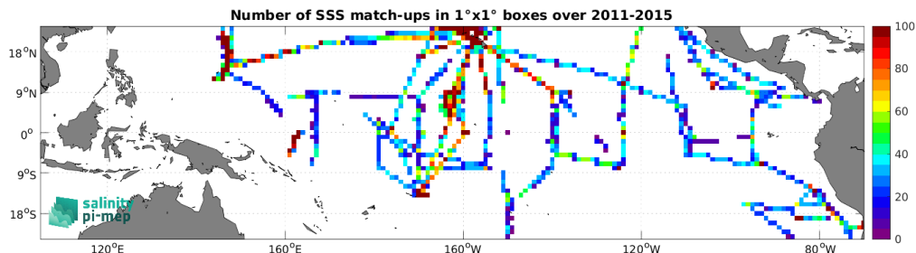
Figure 4: Number of SSS match-ups between TSG (SAMOS) SSS and the Aquarius SSS L3 CAP v5 - Monthly (JPL) SSS product for the Tropical Pacific Ocean Pi-MEP region over 1^\circ \times 1^\circ boxes and for the full satellite product period.
