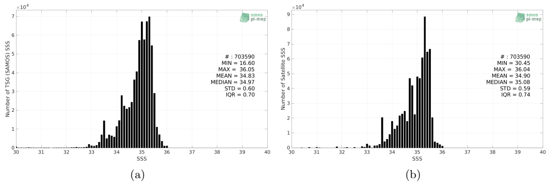
Figure 2: Histograms of SSS from TSG (SAMOS) (a) and Aquarius SSS L3 CAP v5 - Monthly (JPL) (b) considering all match-up pairs per bins of 0.1 over the Tropical Pacific Ocean Pi-MEP region and for the full satellite product period.
