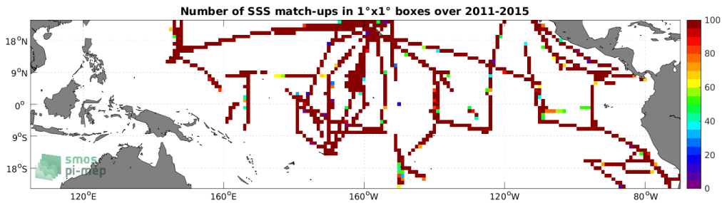
Figure 4: Number of SSS match-ups between TSG (SAMOS) SSS and the Aquarius SSS L3 CAP v5 - Monthly (JPL) SSS product for the Tropical Pacific Ocean Pi-MEP region over 1^\circ \times 1^\circ boxes and for the full satellite product period.
