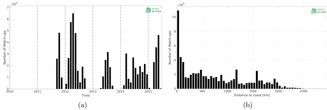
Figure 1: Number of match-ups between TSG (SAMOS) and Aquarius SSS L3 CAP v5 - Monthly (JPL) SSS as a function of time (a) and as function of the distance to coast (b) over the Tropical Pacific Ocean Pi-MEP region and for the full satellite product period.
