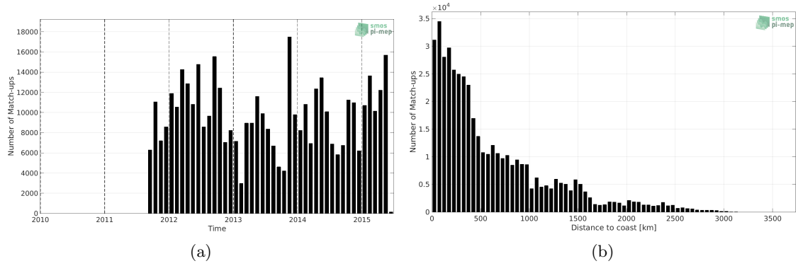
Figure 1: Number of match-ups between TSG (LEGOS-DM) and Aquarius SSS L3 CAP v5 - Monthly (JPL) SSS as a function of time (a) and as function of the distance to coast (b) over the Tropical Pacific Ocean Pi-MEP region and for the full satellite product period.
