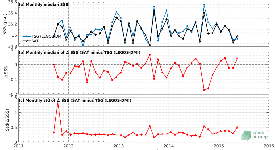
Figure 7: Time series of the monthly median SSS (top), median of \Delta\text{SSS} (Satellite - TSG (LEGOS-DM)) and Std of \Delta\text{SSS} (Satellite - TSG (LEGOS-DM)) over the Tropical Pacific Ocean Pi-MEP region considering all match-ups collected by the Pi-MEP.
