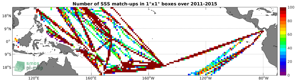
Figure 4: Number of SSS match-ups between TSG (LEGOS-DM) SSS and the Aquarius SSS L3 CAP v5 - Monthly (JPL) SSS product for the Tropical Pacific Ocean Pi-MEP region over 1°x1° boxes and for the full satellite product period.
