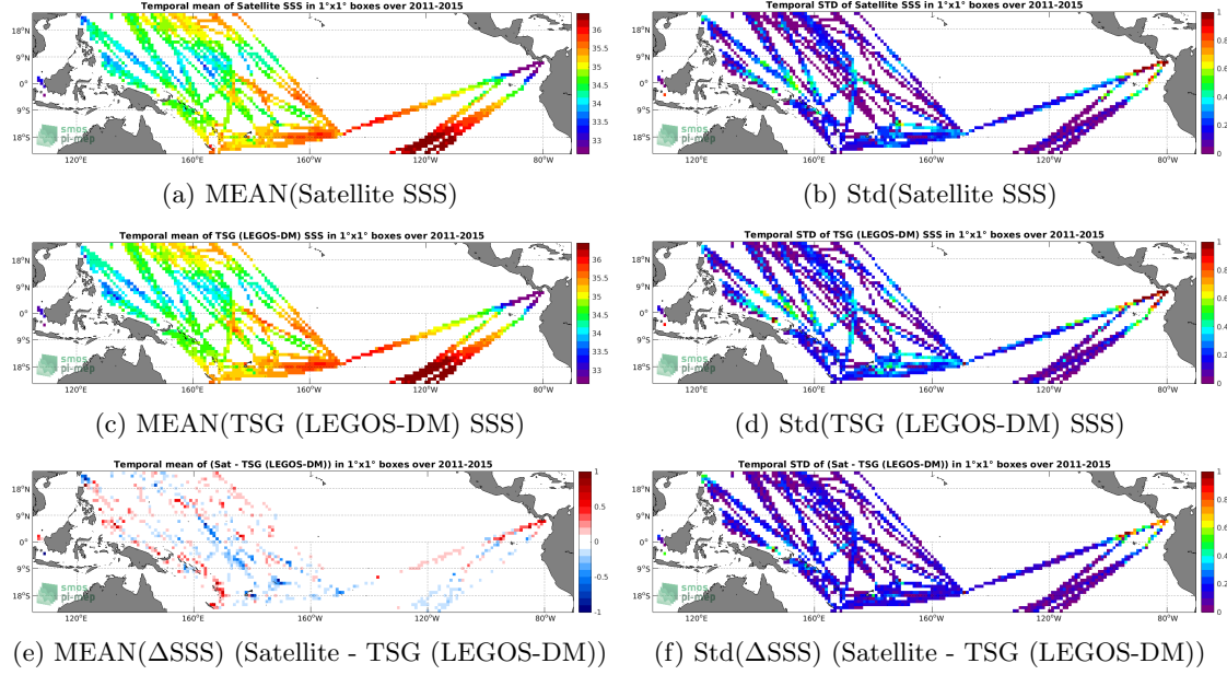
Figure 6: Temporal mean (left) and Std (right) of SSS from Aquarius SSS L3 CAP v5 - Monthly (JPL) (top), TSG (LEGOS-DM) (middle), and of \Delta SSS (Satellite - TSG (LEGOS-DM)). Only match-up pairs are used to generate these maps.
