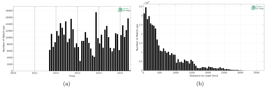
Figure 1: Number of match-ups between TSG-LEGOS-DM and Aquarius-L3-JPL-V5-MONTHLY SSS as a function of time (a) and as function of the distance to coast (b) over the Tropical Pacific Ocean Pi-MEP region and for the full satellite product period.
