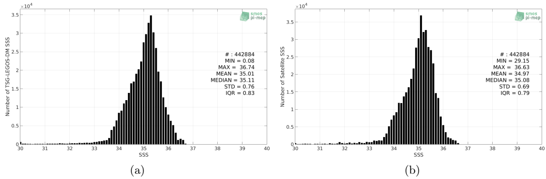
Figure 2: Histograms of SSS from TSG-LEGOS-DM (a) and Aquarius-L3-JPL-V5-MONTHLY (b) considering all match-up pairs per bins of 0.1 over the Tropical Pacific Ocean Pi-MEP region and for the full satellite product period.
