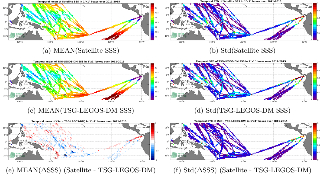
Figure 6: Temporal mean (left) and Std (right) of SSS from Aquarius-L3-JPL-V5-MONTHLY (top), TSG-LEGOS-DM (middle), and of \Delta SSS (Satellite - TSG-LEGOS-DM). Only match-up pairs are used to generate these maps.
