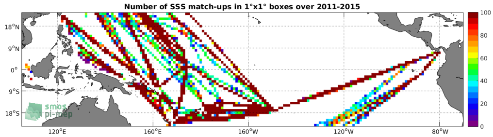
Figure 4: Number of SSS match-ups between TSG-LEGOS-DM SSS and the Aquarius-L3-JPL-V5-MONTHLY SSS product for the Tropical Pacific Ocean Pi-MEP region over 1^\circ \times 1^\circ boxes and for the full satellite product period.
