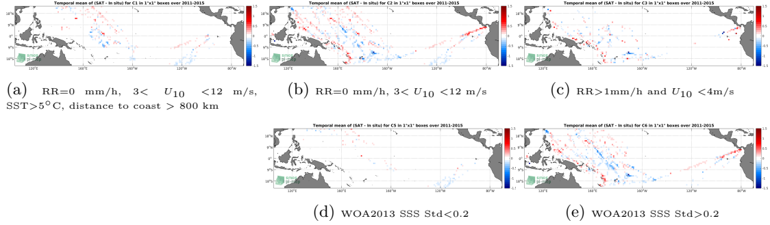
Figure 12: Temporal mean gridded over spatial boxes of size 1^\circ \times 1^\circ of \Delta SSS (Aquarius-L3-JPL-V5-MONTHLY - TSG-LEGOS-DM) for 5 different subdatasets corresponding to:RR=0 mm/h, 3 < U_{10} < 12 m/s, SST >5^\circ\text{C} , distance to coast > 800 km (a), RR=0 mm/h, 3 < U_{10} < 12 m/s (b), RR >1 mm/h and U_{10} < 4 m/s (c), WOA2013 SSS Std <0.2 (d), WOA2013 SSS Std >0.2 (e).
