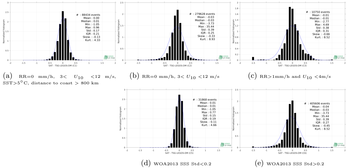
Figure 13: Normalized histogram of \Delta SSS (Aquarius-L3-JPL-V5-MONTHLY - TSG-LEGOS-DM) for 5 different subdatasets corresponding to: RR=0 mm/h, 3 < U_{10} < 12 m/s, SST >5^\circ\text{C} , distance to coast > 800 km (a), RR=0 mm/h, 3 < U_{10} < 12 m/s (b), RR >1 mm/h and U_{10} < 4 m/s (c), WOA2013 SSS Std <0.2 (d), WOA2013 SSS Std >0.2 (e).
