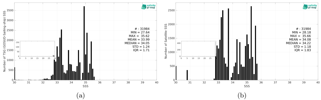
Figure 3: Histograms of SSS from TSG (GOSUD-Sailing-ship) (a) and Aquarius SSS L3 CAP v5 - Monthly (JPL) (b) considering all match-up pairs per bins of 0.1 over the Tropical Pacific Ocean Pi-MEP region and for the full satellite product period.
