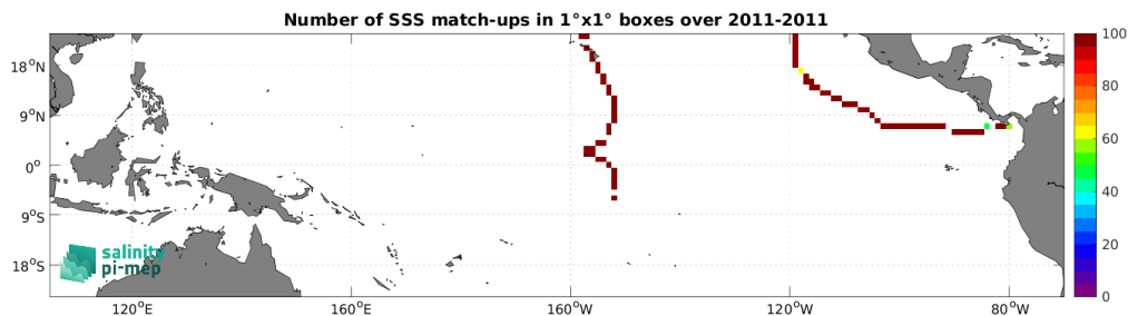
Figure 5: Number of SSS match-ups between TSG (GOSUD-Sailing-ship) SSS and the Aquarius SSS L3 CAP v5 - Monthly (JPL) SSS product for the Tropical Pacific Ocean Pi-MEP region over 1^\circ \times 1^\circ boxes and for the full satellite product period.
