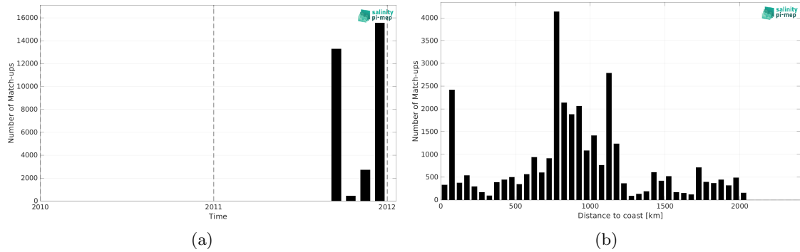
Figure 2: Number of match-ups between TSG (GOSUD-Sailing-ship) and Aquarius SSS L3 CAP v5 - Monthly (JPL) SSS as a function of time (a) and as function of the distance to coast (b) over the Tropical Pacific Ocean Pi-MEP region and for the full satellite product period.
