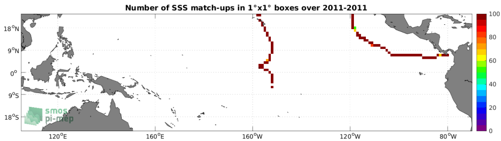
Figure 4: Number of SSS match-ups between TSG (GOSUD-Sailing-ship) SSS and the Aquarius SSS L3 CAP v5 - Monthly (JPL) SSS product for the Tropical Pacific Ocean Pi-MEP region over 1^\circ \times 1^\circ boxes and for the full satellite product period.
