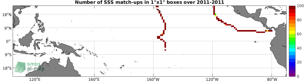
Figure 4: Number of SSS match-ups between TSG (GOSUD-Sailing-ship) SSS and the Aquarius SSS L3 CAP v5 - Monthly (JPL) SSS product for the Tropical Pacific Ocean Pi-MEP region over 1°x1° boxes and for the full satellite product period.
