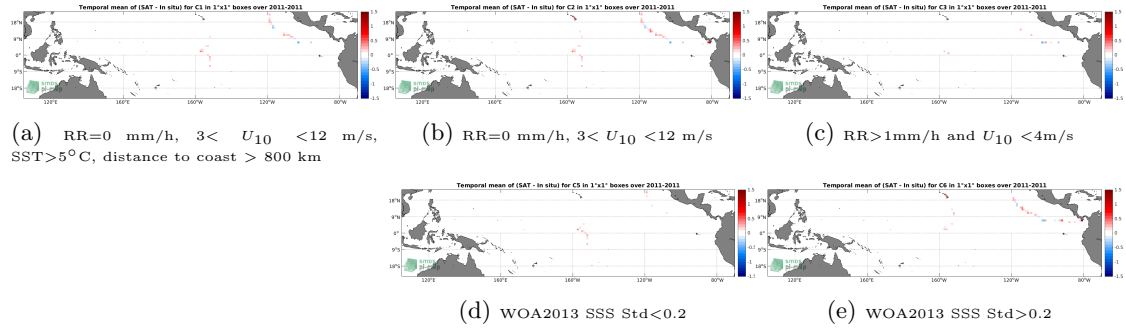
Figure 12: Temporal mean gridded over spatial boxes of size 1^\circ \times 1^\circ of \Delta SSS (Aquarius SSS L3 CAP v5 - Monthly (JPL) - TSG (GOSUD-Sailing-ship)) for 5 different subdatasets corresponding to: RR=0 mm/h, 3 < U_{10} < 12 m/s, SST > 5^\circ C , distance to coast > 800 km (a), RR=0 mm/h, 3 < U_{10} < 12 m/s (b), RR > 1 mm/h and U_{10} < 4 m/s (c), WOA2013 SSS Std < 0.2 (d), WOA2013 SSS Std > 0.2 (e).
