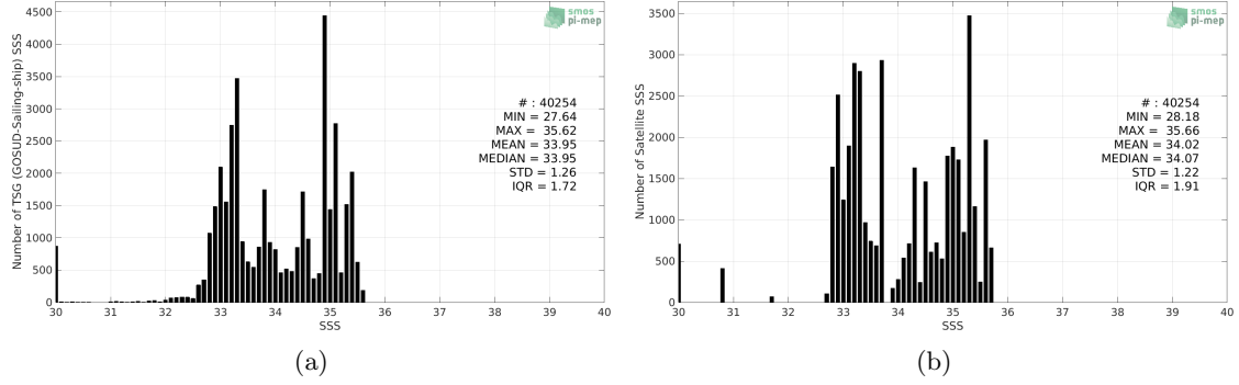
Figure 2: Histograms of SSS from TSG (GOSUD-Sailing-ship) (a) and Aquarius SSS L3 CAP v5 - Monthly (JPL) (b) considering all match-up pairs per bins of 0.1 over the Tropical Pacific Ocean Pi-MEP region and for the full satellite product period.
