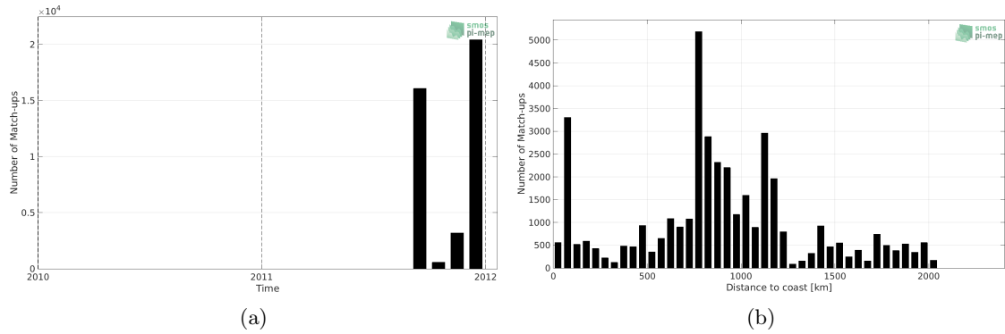
Figure 1: Number of match-ups between TSG (GOSUD-Sailing-ship) and Aquarius SSS L3 CAP v5 - Monthly (JPL) SSS as a function of time (a) and as function of the distance to coast (b) over the Tropical Pacific Ocean Pi-MEP region and for the full satellite product period.
