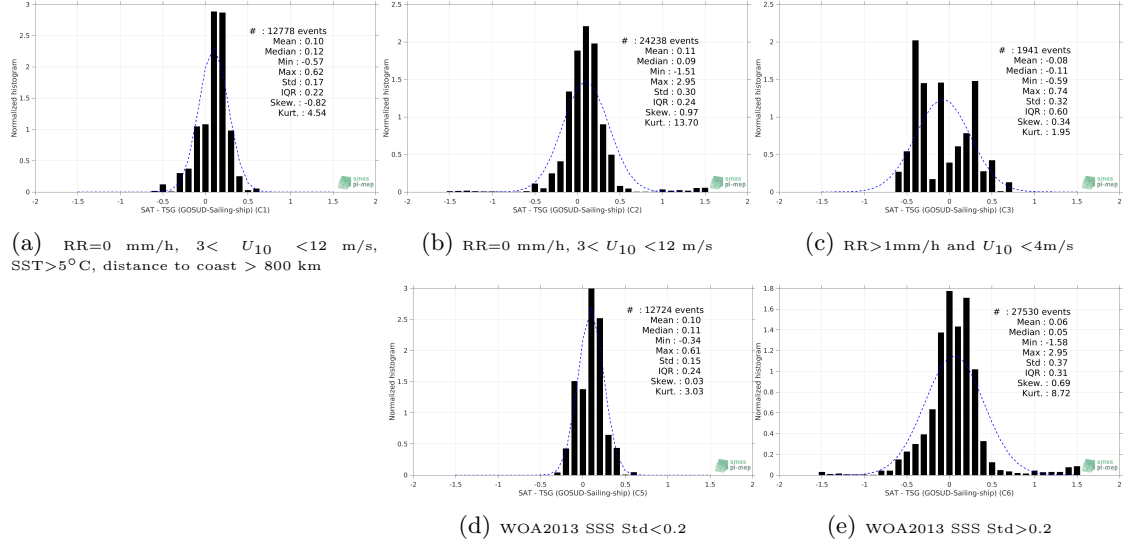
Figure 13: Normalized histogram of \Delta\text{SSS} (Aquarius SSS L3 CAP v5 - Monthly (JPL) - TSG (GOSUD-Sailing-ship)) for 5 different subdatasets corresponding to: RR=0 mm/h, 3 < U_{10} < 12 m/s, SST > 5^\circ\text{C} , distance to coast > 800 km (a), RR=0 mm/h, 3 < U_{10} < 12 m/s (b), RR > 1\text{mm/h} and U_{10} < 4\text{m/s} (c), WOA2013 SSS Std < 0.2 (d), WOA2013 SSS Std > 0.2 (e).
