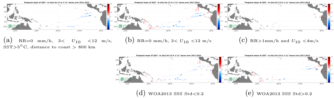
Figure 12: Temporal mean gridded over spatial boxes of size 1^{\circ}\times 1^{\circ} of \Delta SSS (Aquarius SSS L3 CAP v5 - Monthly (JPL) - TSG (GOSUD-Research-vessel)) for 5 different subdatasets corresponding to: RR=0 mm/h, 3 < U_{10} < 12 m/s, SST > 5^{\circ}\text{C} , distance to coast > 800 km (a), RR=0 mm/h, 3 < U_{10} < 12 m/s (b), RR > 1 mm/h and U_{10} < 4 m/s (c), WOA2013 SSS Std < 0.2 (d), WOA2013 SSS Std > 0.2 (e).
