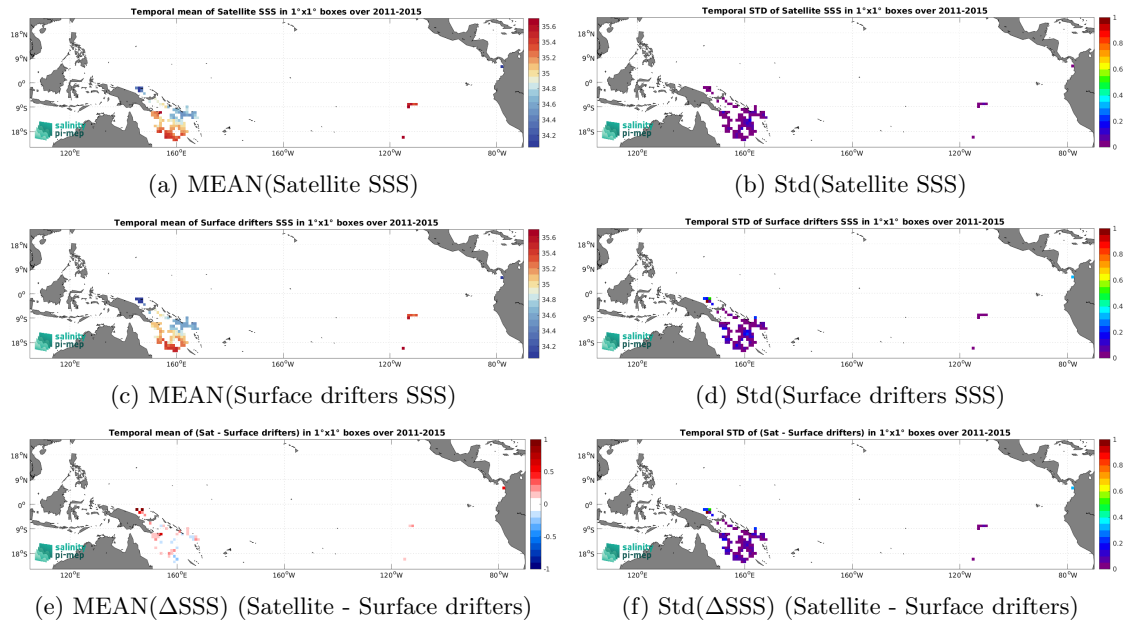
Figure 6: Temporal mean (left) and Std (right) of SSS from Aquarius SSS L3 CAP v5 - Monthly (JPL) (top), Surface drifters (middle), and of \Delta SSS (Satellite - Surface drifters). Only match-up pairs are used to generate these maps.
