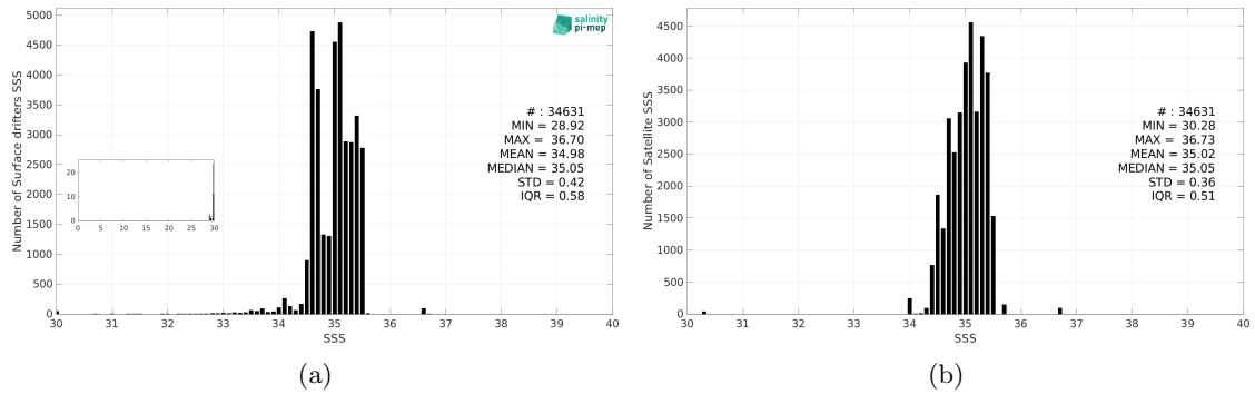
Figure 3: Histograms of SSS from Surface drifters (a) and Aquarius SSS L3 CAP v5 - Monthly (JPL) (b) considering all match-up pairs per bins of 0.1 over the Tropical Pacific Ocean Pi-MEP region and for the full satellite product period.
