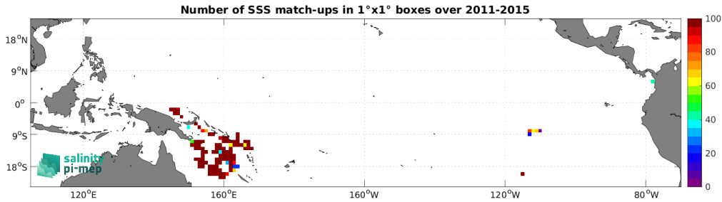
Figure 4: Number of SSS match-ups between Surface drifters SSS and the Aquarius SSS L3 CAP v5 - Monthly (JPL) SSS product for the Tropical Pacific Ocean Pi-MEP region over 1^\circ \times 1^\circ boxes and for the full satellite product period.
