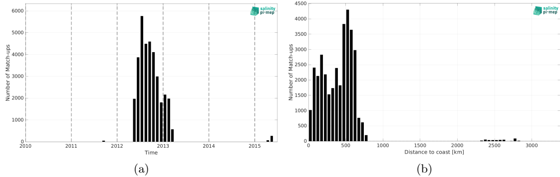
Figure 2: Number of match-ups between Surface drifters and Aquarius SSS L3 CAP v5 - Monthly (JPL) SSS as a function of time (a) and as function of the distance to coast (b) over the Tropical Pacific Ocean Pi-MEP region and for the full satellite product period.
