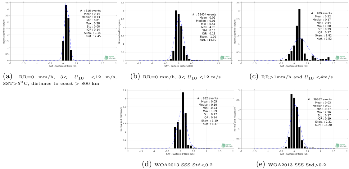
Figure 12: Normalized histogram of \Delta SSS (Aquarius-L3-JPL-V5-MONTHLY - Surface drifters) for 5 different subdatasets corresponding to: RR=0 mm/h, 3 < U_{10} < 12 m/s, SST > 5^\circ C , distance to coast > 800 km (a), RR=0 mm/h, 3 < U_{10} < 12 m/s (b), RR > 1 mm/h and U_{10} < 4 m/s (c), WOA2013 SSS Std < 0.2 (d), WOA2013 SSS Std > 0.2 (e).
