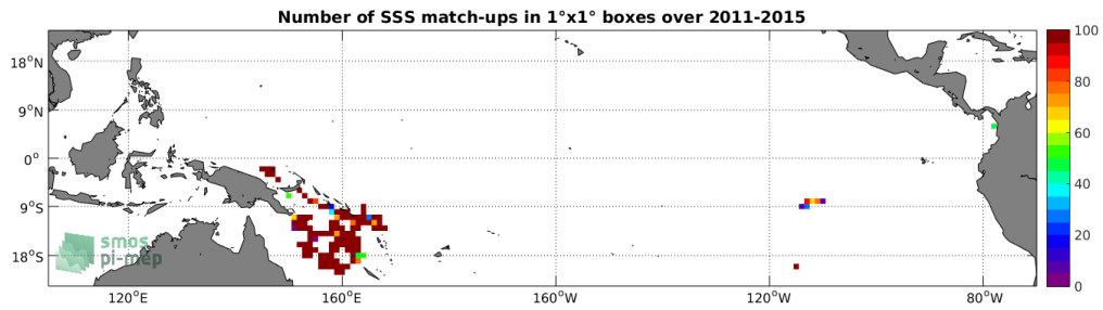
Figure 3: Number of SSS match-ups between Surface drifters SSS and the Aquarius-L3-JPL-V5-MONTHLY SSS product for the Tropical Pacific Ocean Pi-MEP region over 1^\circ \times 1^\circ boxes and for the full satellite product period.
