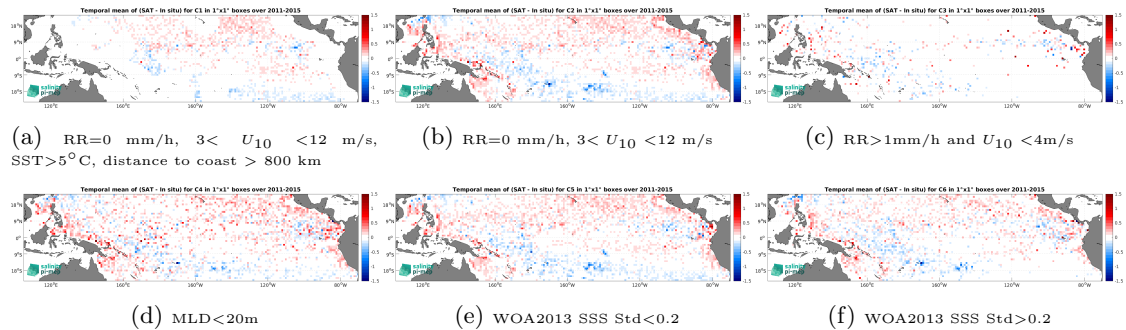
Figure 14: Temporal mean gridded over spatial boxes of size 1^\circ \times 1^\circ of \Delta\text{SSS} (Aquarius SSS L3 CAP v5 - Monthly (JPL) - Argo) for 6 different subdatasets corresponding to: RR=0 mm/h, 3 < U_{10} < 12 m/s, SST > 5°C, distance to coast > 800 km (a), RR=0 mm/h, 3 < U_{10} < 12 m/s (b), RR > 1mm/h and U_{10} < 4 m/s (c), MLD < 20m (d), WOA2013 SSS Std < 0.2 (e), WOA2013 SSS Std > 0.2 (f).
