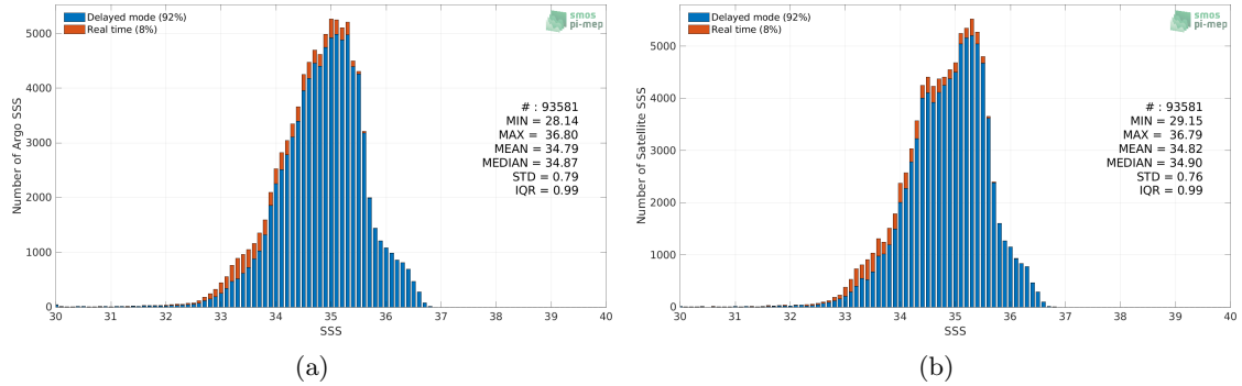
Figure 2: Histograms of SSS from Argo (a) and Aquarius SSS L3 CAP v5 - Monthly (JPL) (b) considering all match-up pairs per bins of 0.1 over the Tropical Pacific Ocean Pi-MEP region and for the full satellite product period.
