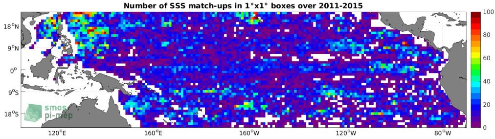
Figure 4: Number of SSS match-ups between Argo SSS and the Aquarius SSS L3 CAP v5 - Monthly (JPL) SSS product for the Tropical Pacific Ocean Pi-MEP region over 1^\circ \times 1^\circ boxes and for the full satellite product period.
