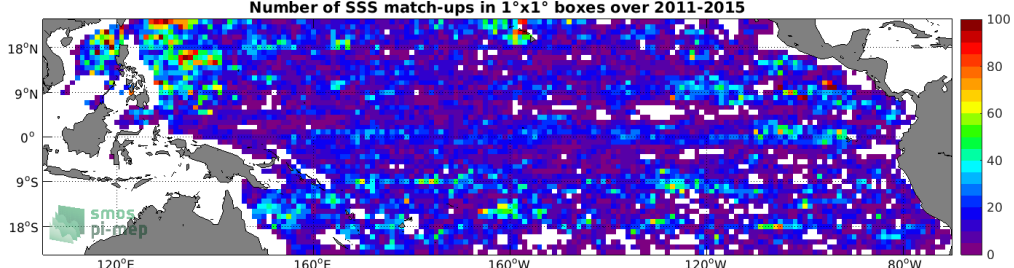
Figure 4: Number of SSS match-ups between Argo SSS and the Aquarius SSS L3 CAP v5 - Monthly (JPL) SSS product for the Tropical Pacific Ocean Pi-MEP region over 1^\circ \times 1^\circ boxes and for the full satellite product period.
