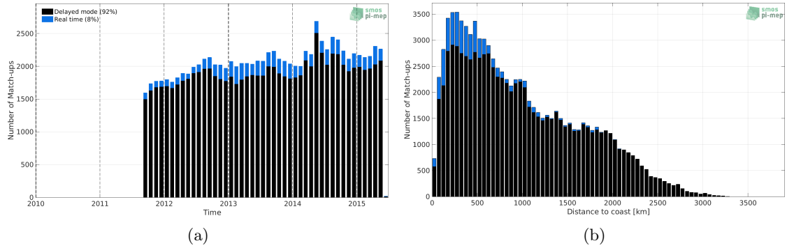
Figure 1: Number of match-ups between Argo and Aquarius SSS L3 CAP v5 - Monthly (JPL) SSS as a function of time (a) and as function of the distance to coast (b) over the Tropical Pacific Ocean Pi-MEP region and for the full satellite product period.
