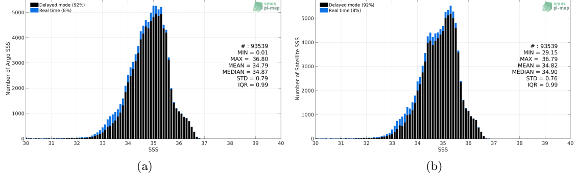
Figure 2: Histograms of SSS from Argo (a) and Aquarius SSS L3 CAP v5 - Monthly (JPL) (b) considering all match-up pairs per bins of 0.1 over the Tropical Pacific Ocean Pi-MEP region and for the full satellite product period.
