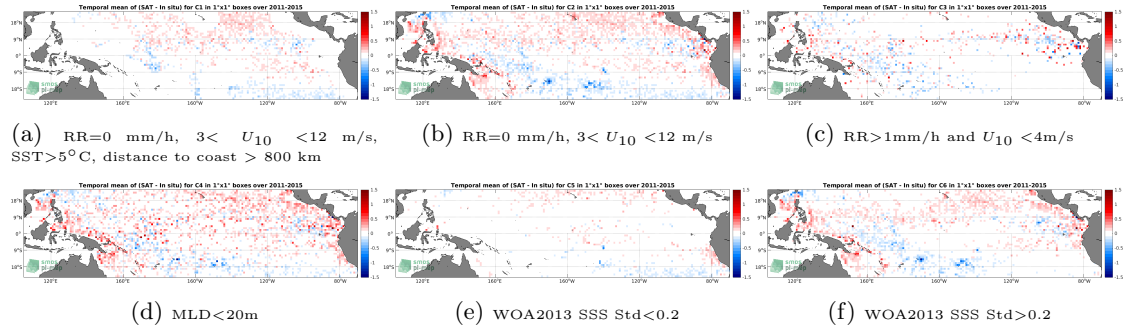
Figure 12: Temporal mean gridded over spatial boxes of size 1^\circ \times 1^\circ of \Delta SSS (Aquarius SSS L3 CAP v5 - Monthly (JPL) - Argo) for 6 different subdatasets corresponding to: RR=0 mm/h, 3 < U_{10} < 12 m/s, SST > 5^\circ\text{C} , distance to coast > 800 km (a), RR=0 mm/h, 3 < U_{10} < 12 m/s (b), RR > 1 mm/h and U_{10} < 4 m/s (c), MLD < 20 m (d), WOA2013 SSS Std < 0.2 (e), WOA2013 SSS Std > 0.2 (f).
