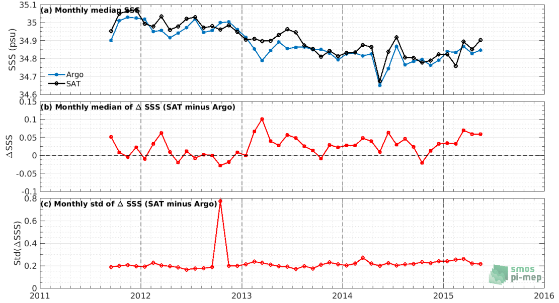
Figure 7: Time series of the monthly median SSS (top), median of \Delta\text{SSS} (Satellite - Argo) and Std of \Delta\text{SSS} (Satellite - Argo) over the Tropical Pacific Ocean Pi-MEP region considering all match-ups collected by the Pi-MEP.
