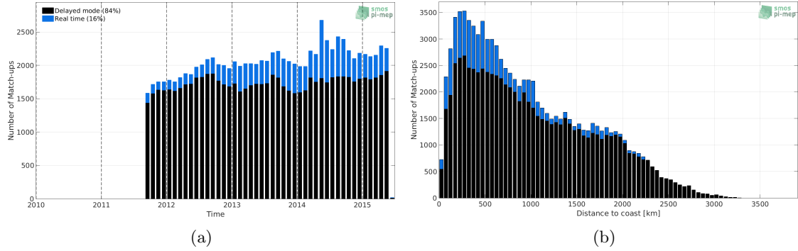
Figure 1: Number of match-ups between Argo and Aquarius-L3-JPL-V5-MONTHLY SSS as a function of time (a) and as function of the distance to coast (b) over the Tropical Pacific Ocean Pi-MEP region and for the full satellite product period.
