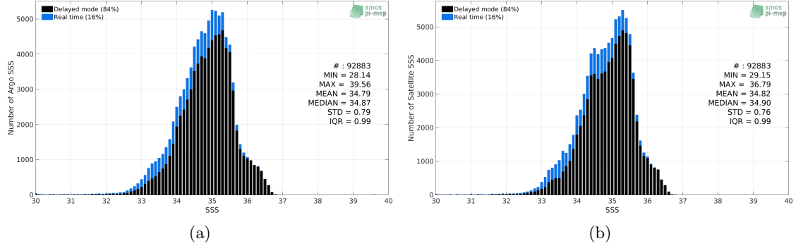
Figure 2: Histograms of SSS from Argo (a) and Aquarius-L3-JPL-V5-MONTHLY (b) considering all match-up pairs per bins of 0.1 over the Tropical Pacific Ocean Pi-MEP region and for the full satellite product period.
