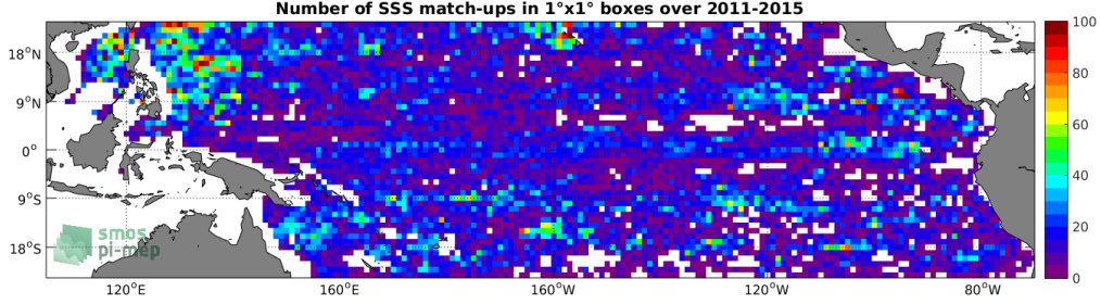
Figure 4: Number of SSS match-ups between Argo SSS and the Aquarius-L3-JPL-V5-MONTHLY SSS product for the Tropical Pacific Ocean Pi-MEP region over 1^\circ \times 1^\circ boxes and for the full satellite product period.
