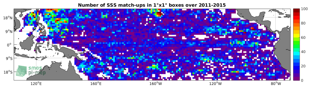
Figure 4: Number of SSS match-ups between Argo SSS and the Aquarius-L3-JPL-V5-MONTHLY SSS product for the Tropical Pacific Ocean Pi-MEP region over 1°x1° boxes and for the full satellite product period.
