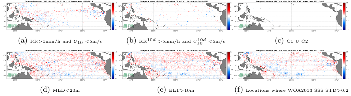
Figure 12: Temporal mean gridded over spatial boxes of size 1^\circ \times 1^\circ of \Delta\text{SSS} (Aquarius-L3-JPL-V5-MONTHLY - Argo) for 6 different subdatasets corresponding to: \text{RR} > 1\text{mm/h} and U_{10} < 5\text{m/s} (a), \text{RR}^{10d} > 5\text{mm/h} and U_{10}^{10d} < 5\text{m/s} (b), C1 U C2 (c), \text{MLD} < 20\text{m} (d), \text{BLT} > 10\text{m} (e), Locations where WOA2013 SSS STD > 0.2 (f).
