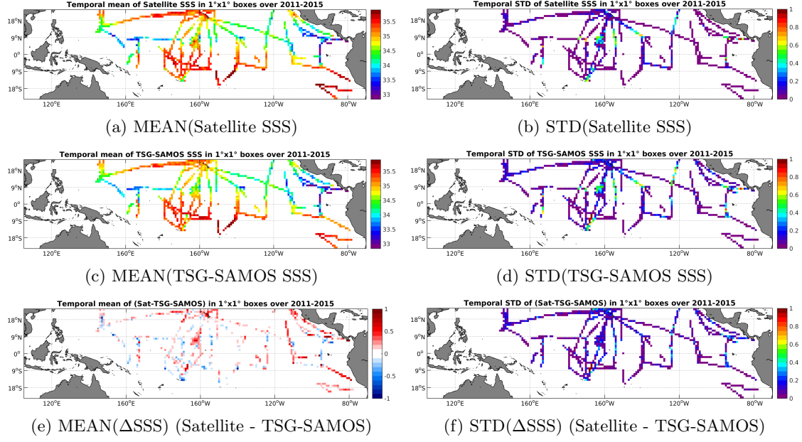
Figure 6: Temporal mean (left) and STD (right) of SSS from Aquarius-L3-JPL-V4-7DAY-RUNNING (top), TSG-SAMOS (middle), and of \Delta SSS (Satellite - TSG-SAMOS). Only match-up pairs are used to generate these maps.
