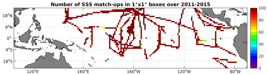
Figure 4: Number of SSS match-ups between TSG-SAMOS SSS and the Aquarius-L3-JPL-V4-7DAY-RUNNING SSS product for the Tropical Pacific Ocean Pi-MEP region over 1^\circ \times 1^\circ boxes and for the full satellite product period.
