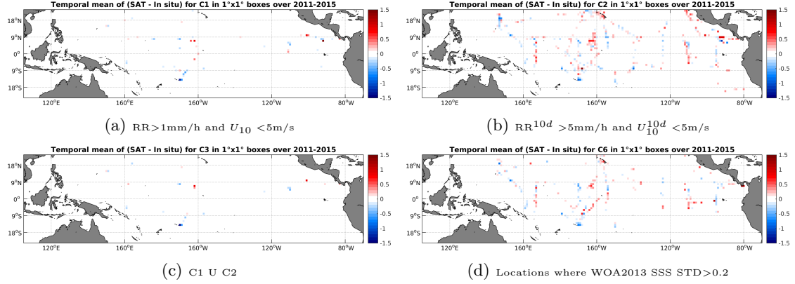
Figure 12: Temporal mean gridded over spatial boxes of size 1^\circ \times 1^\circ of \Delta SSS (Aquarius-L3-JPL-V4-7DAY-RUNNING - TSG-SAMOS) for 4 different subdatasets corresponding to: RR > 1 mm/h and U_{10} < 5 m/s (a), RR 10d > 5 mm/h and U_{10}^{10d} < 5 m/s (b), C1 U C2 (c), Locations where WOA2013 SSS STD > 0.2 (d).
