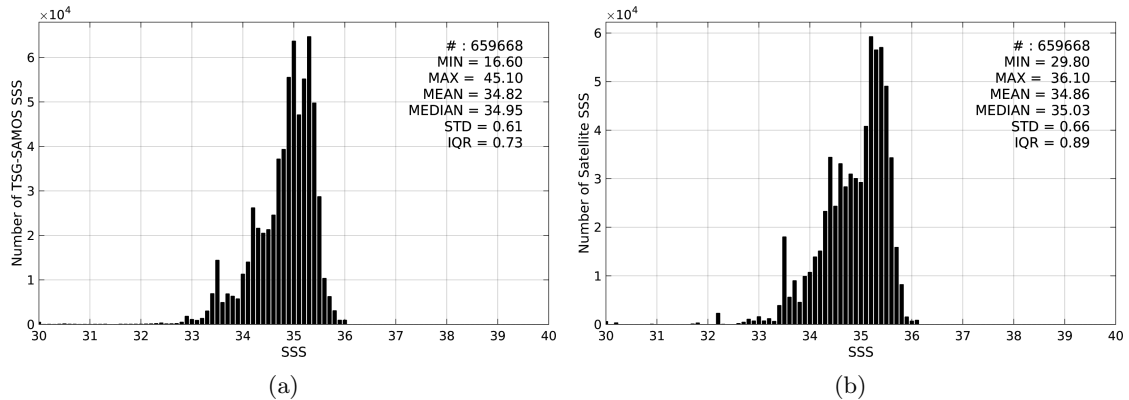
Figure 2: Histograms of SSS from TSG-SAMOS (a) and Aquarius-L3-JPL-V4-7DAY-RUNNING (b) considering all match-up pairs per bins of 0.1 over the Tropical Pacific Ocean Pi-MEP region and for the full satellite product period.
