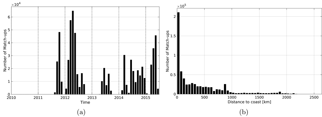
Figure 1: Number of match-ups between TSG-SAMOS and Aquarius-L3-JPL-V4-7DAY-RUNNING SSS as a function of time (a) and as function of the distance to coast (b) over the Tropical Pacific Ocean Pi-MEP region and for the full satellite product period.
