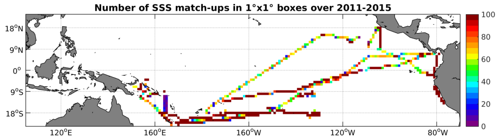
Figure 4: Number of SSS match-ups between TSG-GOSUD-Research-vessel SSS and the Aquarius-L3-JPL-V4-7DAY-RUNNING SSS product for the Tropical Pacific Ocean Pi-MEP region over 1^\circ \times 1^\circ boxes and for the full satellite product period.
