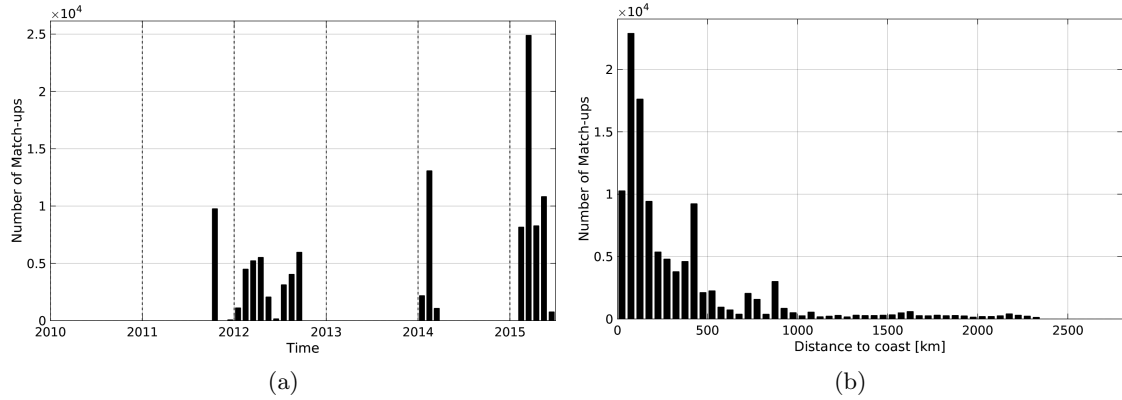
Figure 1: Number of match-ups between TSG-GOSUD-Research-vessel and Aquarius-L3-JPL-V4-7DAY-RUNNING SSS as a function of time (a) and as function of the distance to coast (b) over the Tropical Pacific Ocean Pi-MEP region and for the full satellite product period.
