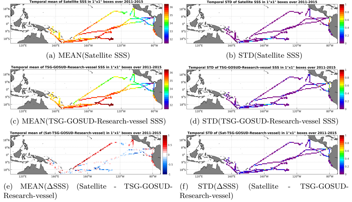
Figure 6: Temporal mean (left) and STD (right) of SSS from Aquarius-L3-JPL-V4-7DAY-RUNNING (top), TSG-GOSUD-Research-vessel (middle), and of \Delta SSS (Satellite - TSG-GOSUD-Research-vessel). Only match-up pairs are used to generate these maps.
