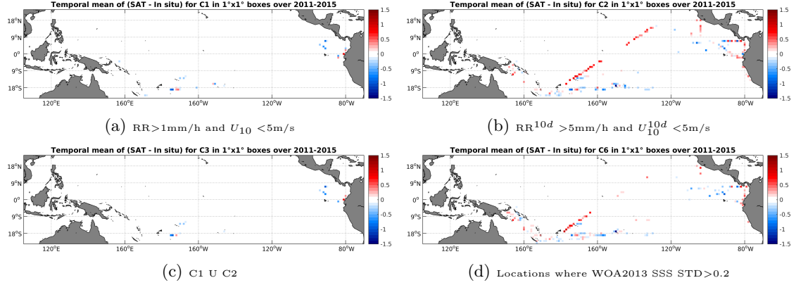
Figure 12: Temporal mean gridded over spatial boxes of size 1^\circ \times 1^\circ of \Delta SSS (Aquarius-L3-JPL-V4-7DAY-RUNNING - TSG-GOSUD-Research-vessel) for 4 different subdatasets corresponding to: RR > 1\text{mm/h} and U_{10} < 5\text{m/s} (a), RR^{10d} > 5\text{mm/h} and U_{10}^{10d} < 5\text{m/s} (b), C1 U C2 (c), Locations where WOA2013 SSS STD > 0.2 (d).
