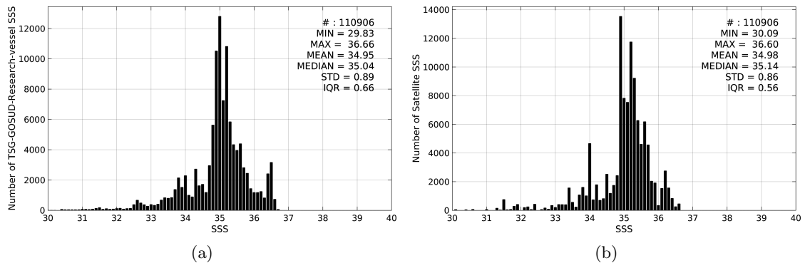
Figure 2: Histograms of SSS from TSG-GOSUD-Research-vessel (a) and Aquarius-L3-JPL-V4-7DAY-RUNNING (b) considering all match-up pairs per bins of 0.1 over the Tropical Pacific Ocean Pi-MEP region and for the full satellite product period.
