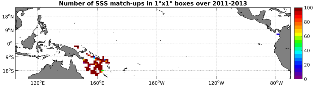
Figure 3: Number of SSS match-ups between Surface drifters SSS and the Aquarius-L3-JPL-V4-7DAY-RUNNING SSS product for the Tropical Pacific Ocean Pi-MEP region over 1^\circ \times 1^\circ boxes and for the full satellite product period.
