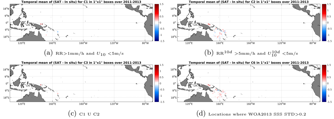
Figure 11: Temporal mean gridded over spatial boxes of size 1^\circ \times 1^\circ of \Delta SSS (Aquarius-L3-JPL-V4-7DAY-RUNNING - Surface drifters) for 4 different subdatasets corresponding to: RR > 1 mm/h and U_{10} < 5 m/s (a), RR^{10d} > 5 mm/h and U_{10}^{10d} < 5 m/s (b), C1 U C2 (c), Locations where WOA2013 SSS STD > 0.2 (d).
