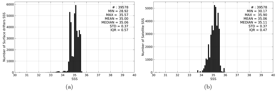
Figure 2: Histograms of SSS from Surface drifters (a) and Aquarius-L3-JPL-V4-7DAY-RUNNING (b) considering all match-up pairs per bins of 0.1 over the Tropical Pacific Ocean Pi-MEP region and for the full satellite product period.
