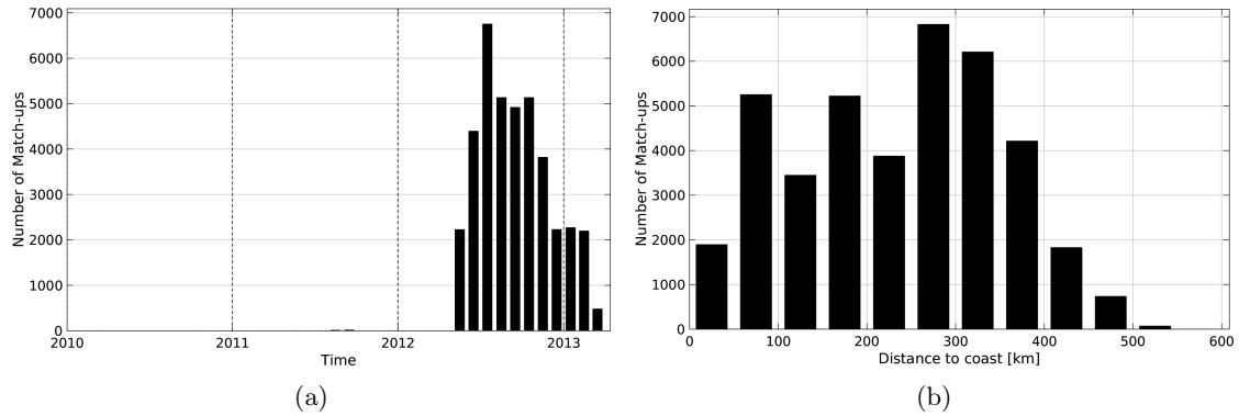
Figure 1: Number of match-ups between Surface drifters and Aquarius-L3-JPL-V4-7DAY-RUNNING SSS as a function of time (a) and as function of the distance to coast (b) over the Tropical Pacific Ocean Pi-MEP region and for the full satellite product period.
