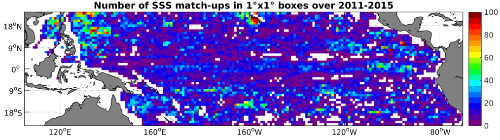
Figure 4: Number of SSS match-ups between Argo SSS and the Aquarius-L3-JPL-V4-7DAY-RUNNING SSS product for the Tropical Pacific Ocean Pi-MEP region over 1^\circ \times 1^\circ boxes and for the full satellite product period.
