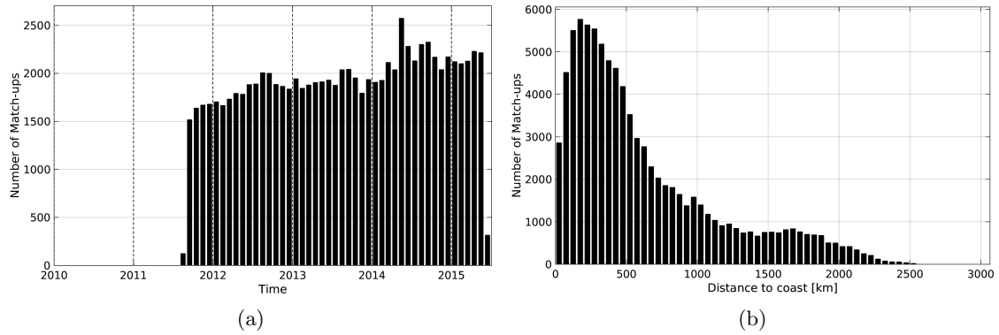
Figure 1: Number of match-ups between Argo and Aquarius-L3-JPL-V4-7DAY-RUNNING SSS as a function of time (a) and as function of the distance to coast (b) over the Tropical Pacific Ocean Pi-MEP region and for the full satellite product period.
