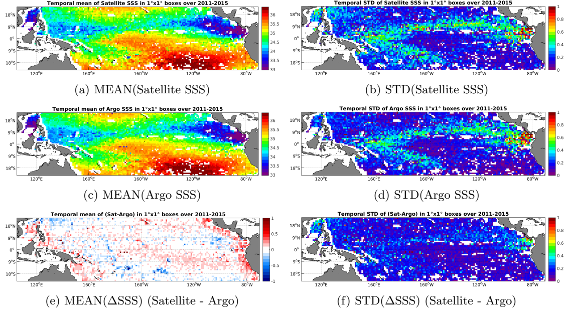
Figure 6: Temporal mean (left) and STD (right) of SSS from Aquarius-L3-JPL-V4-7DAY-RUNNING (top), Argo (middle), and of \Delta SSS (Satellite - Argo). Only match-up pairs are used to generate these maps.
