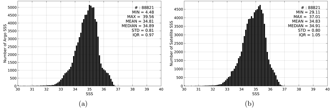
Figure 2: Histograms of SSS from Argo (a) and Aquarius-L3-JPL-V4-7DAY-RUNNING (b) considering all match-up pairs per bins of 0.1 over the Tropical Pacific Ocean Pi-MEP region and for the full satellite product period.
