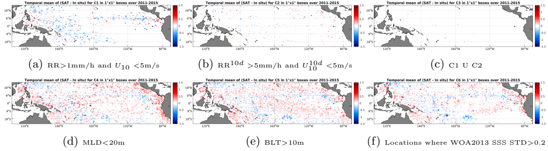
Figure 12: Temporal mean gridded over spatial boxes of size 1^\circ \times 1^\circ of \Delta SSS (Aquarius-L3-JPL-V4-7DAY-RUNNING - Argo) for 6 different subdatasets corresponding to: RR > 1\text{mm/h} and U_{10} < 5\text{m/s} (a), RR^{10d} > 5\text{mm/h} and U_{10}^{10d} < 5\text{m/s} (b), C1 U C2 (c), MLD < 20\text{m} (d), BLT > 10\text{m} (e), Locations where WOA2013 SSS STD > 0.2 (f).
