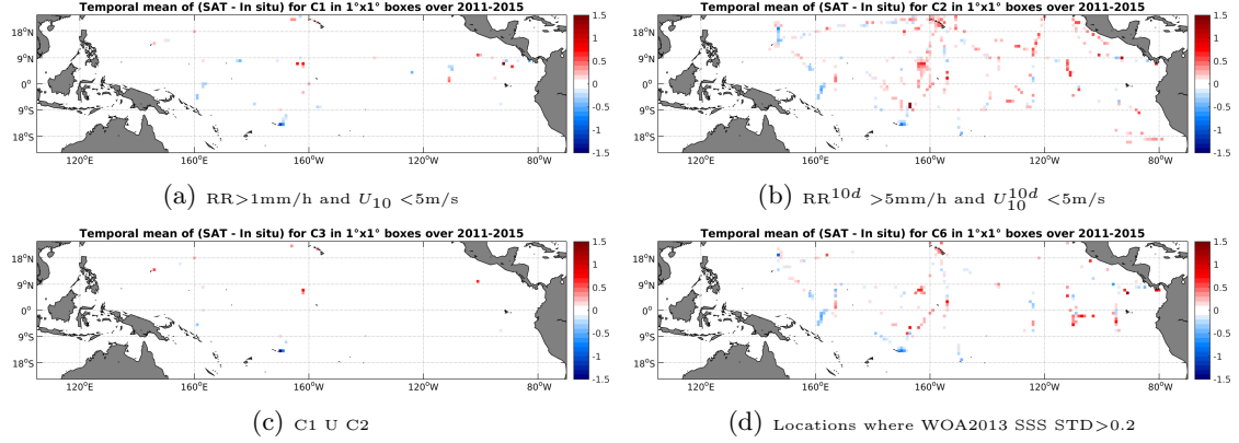
Figure 12: Temporal mean gridded over spatial boxes of size 1^\circ \times 1^\circ of \Delta SSS (Aquarius-L3-JPL-V4-MONTHLY - TSG-SAMOS) for 4 different subdatasets corresponding to: RR > 1\text{mm/h} and U_{10} < 5\text{m/s} (a), RR^{10d} > 5\text{mm/h} and U_{10}^{10d} < 5\text{m/s} (b), C1 U C2 (c), Locations where WOA2013 SSS STD > 0.2 (d).
