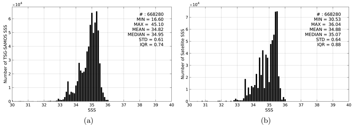
Figure 2: Histograms of SSS from TSG-SAMOS (a) and Aquarius-L3-JPL-V4-MONTHLY (b) considering all match-up pairs per bins of 0.1 over the Tropical Pacific Ocean Pi-MEP region and for the full satellite product period.
