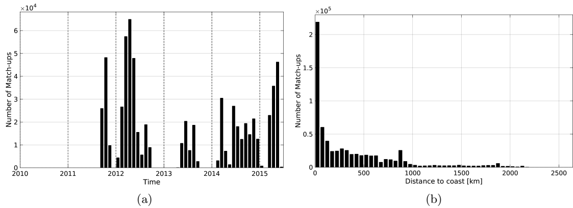
Figure 1: Number of match-ups between TSG-SAMOS and Aquarius-L3-JPL-V4-MONTHLY SSS as a function of time (a) and as function of the distance to coast (b) over the Tropical Pacific Ocean Pi-MEP region and for the full satellite product period.
