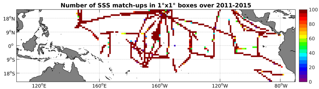
Figure 4: Number of SSS match-ups between TSG-SAMOS SSS and the Aquarius-L3-JPL-V4-MONTHLY SSS product for the Tropical Pacific Ocean Pi-MEP region over 1^\circ \times 1^\circ boxes and for the full satellite product period.
