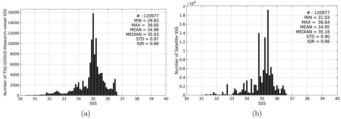
Figure 2: Histograms of SSS from TSG-GOSUD-Research-vessel (a) and Aquarius-L3-JPL-V4-MONTHLY (b) considering all match-up pairs per bins of 0.1 over the Tropical Pacific Ocean Pi-MEP region and for the full satellite product period.
