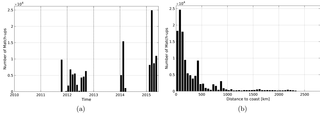
Figure 1: Number of match-ups between TSG-GOSUD-Research-vessel and Aquarius-L3-JPL-V4-MONTHLY SSS as a function of time (a) and as function of the distance to coast (b) over the Tropical Pacific Ocean Pi-MEP region and for the full satellite product period.
