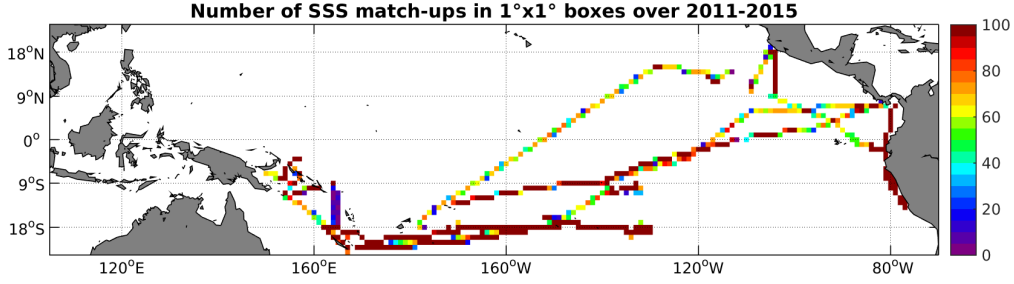
Figure 4: Number of SSS match-ups between TSG-GOSUD-Research-vessel SSS and the Aquarius-L3-JPL-V4-MONTHLY SSS product for the Tropical Pacific Ocean Pi-MEP region over 1^\circ \times 1^\circ boxes and for the full satellite product period.
