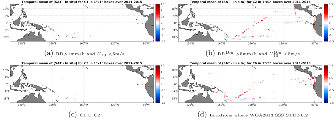
Figure 12: Temporal mean gridded over spatial boxes of size 1^\circ \times 1^\circ of \Delta SSS (Aquarius-L3-JPL-V4-MONTHLY - TSG-GOSUD-Research-vessel) for 4 different subdatasets corresponding to: RR > 1 mm/h and U_{10} < 5 m/s (a), RR 10d > 5 mm/h and U_{10}^{10d} < 5 m/s (b), C1 U C2 (c), Locations where WOA2013 SSS STD > 0.2 (d).
