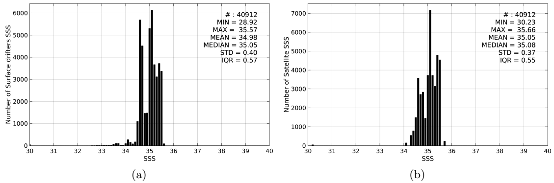
Figure 2: Histograms of SSS from Surface drifters (a) and Aquarius-L3-JPL-V4-MONTHLY (b) considering all match-up pairs per bins of 0.1 over the Tropical Pacific Ocean Pi-MEP region and for the full satellite product period.
