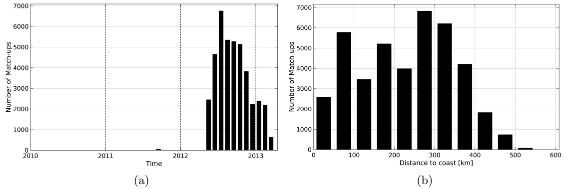
Figure 1: Number of match-ups between Surface drifters and Aquarius-L3-JPL-V4-MONTHLY SSS as a function of time (a) and as function of the distance to coast (b) over the Tropical Pacific Ocean Pi-MEP region and for the full satellite product period.
