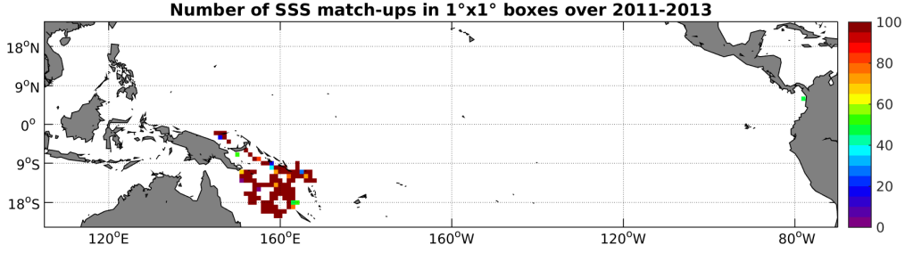
Figure 3: Number of SSS match-ups between Surface drifters SSS and the Aquarius-L3-JPL-V4-MONTHLY SSS product for the Tropical Pacific Ocean Pi-MEP region over 1^\circ \times 1^\circ boxes and for the full satellite product period.
