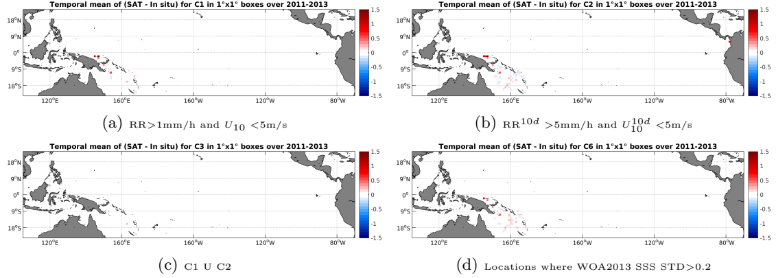
Figure 11: Temporal mean gridded over spatial boxes of size 1^\circ \times 1^\circ of \Delta SSS (Aquarius-L3-JPL-V4-MONTHLY - Surface drifters) for 4 different subdatasets corresponding to: RR > 1\text{mm/h} and U_{10} < 5\text{m/s} (a), RR^{10d} > 5\text{mm/h} and U_{10}^{10d} < 5\text{m/s} (b), C1 U C2 (c), Locations where WOA2013 SSS STD > 0.2 (d).
