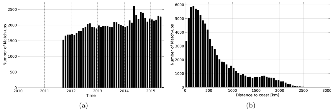
Figure 1: Number of match-ups between Argo and Aquarius-L3-JPL-V4-MONTHLY SSS as a function of time (a) and as function of the distance to coast (b) over the Tropical Pacific Ocean Pi-MEP region and for the full satellite product period.
