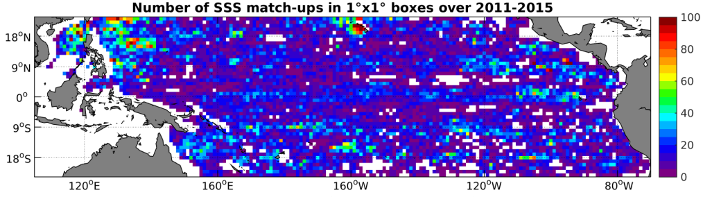
Figure 4: Number of SSS match-ups between Argo SSS and the Aquarius-L3-JPL-V4-MONTHLY SSS product for the Tropical Pacific Ocean Pi-MEP region over 1^\circ \times 1^\circ boxes and for the full satellite product period.
