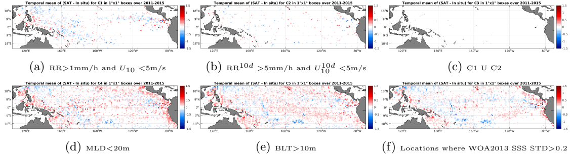
Figure 12: Temporal mean gridded over spatial boxes of size 1^\circ \times 1^\circ of \Delta SSS (Aquarius-L3-JPL-V4-MONTHLY - Argo) for 6 different subdatasets corresponding to: RR > 1\text{mm/h} and U_{10} < 5\text{m/s} (a), RR^{10d} > 5\text{mm/h} and U_{10}^{10d} < 5\text{m/s} (b), C1 U C2 (c), MLD < 20\text{m} (d), BLT > 10\text{m} (e), Locations where WOA2013 SSS STD > 0.2 (f).
