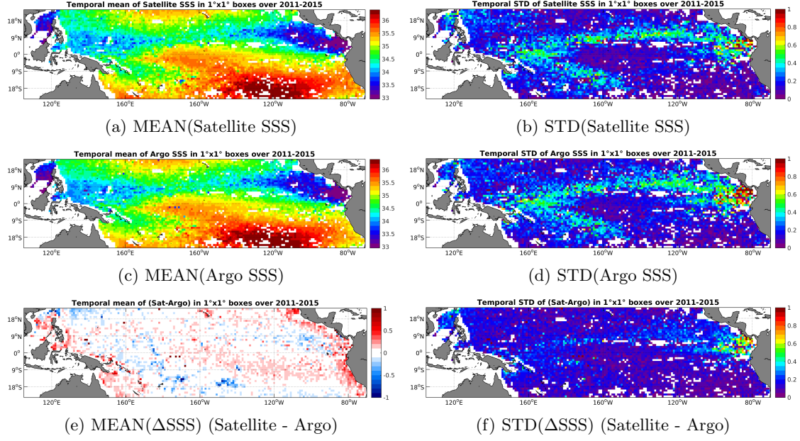
Figure 6: Temporal mean (left) and STD (right) of SSS from Aquarius-L3-JPL-V4-MONTHLY (top), Argo (middle), and of \Delta SSS (Satellite - Argo). Only match-up pairs are used to generate these maps.
