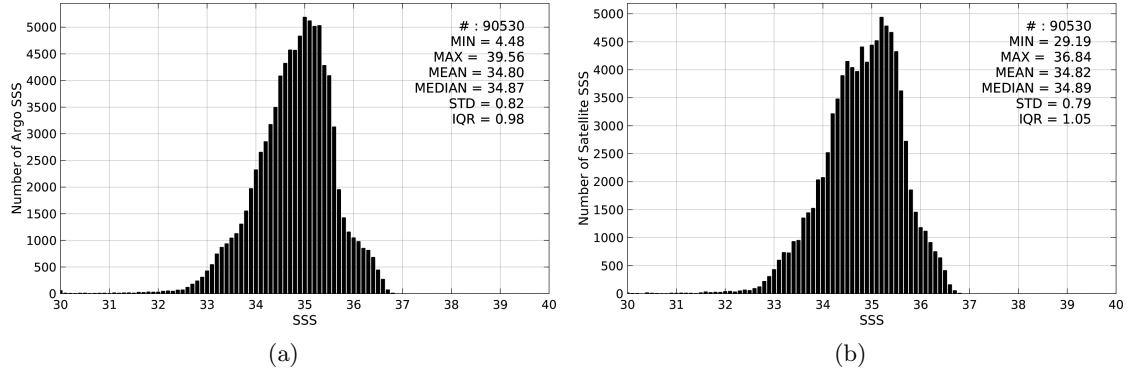
Figure 2: Histograms of SSS from Argo (a) and Aquarius-L3-JPL-V4-MONTHLY (b) considering all match-up pairs per bins of 0.1 over the Tropical Pacific Ocean Pi-MEP region and for the full satellite product period.
