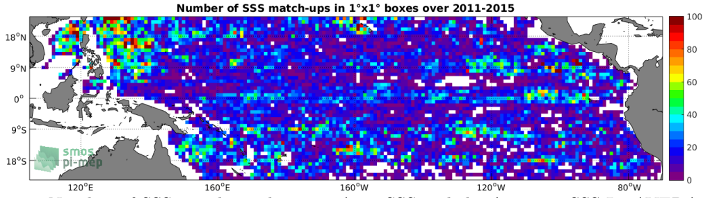
Figure 4: Number of SSS match-ups between Argo SSS and the Aquarius SSS L2-AVERAGED OR v5 (NASA-GSFC) SSS product for the Tropical Pacific Ocean Pi-MEP region over 1^\circ \times 1^\circ boxes and for the full satellite product period.
