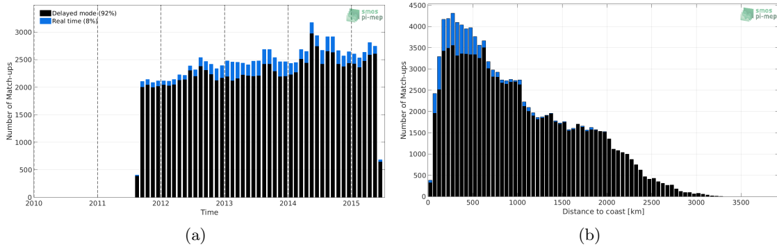
Figure 1: Number of match-ups between Argo and Aquarius SSS L2-AVERAGED OR v5 (NASA-GSFC) SSS as a function of time (a) and as function of the distance to coast (b) over the Tropical Pacific Ocean Pi-MEP region and for the full satellite product period.
