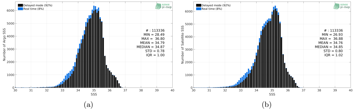
Figure 2: Histograms of SSS from Argo (a) and Aquarius SSS L2-AVERAGED OR v5 (NASA-GSFC) (b) considering all match-up pairs per bins of 0.1 over the Tropical Pacific Ocean Pi-MEP region and for the full satellite product period.
