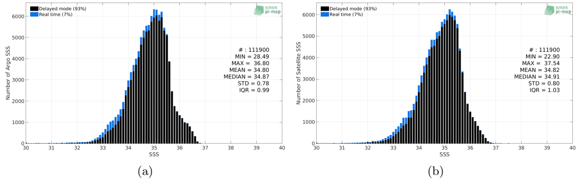
Figure 2: Histograms of SSS from Argo (a) and Aquarius SSS L2-AVERAGED CAP v5 (JPL) (b) considering all match-up pairs per bins of 0.1 over the Tropical Pacific Ocean Pi-MEP region and for the full satellite product period.
