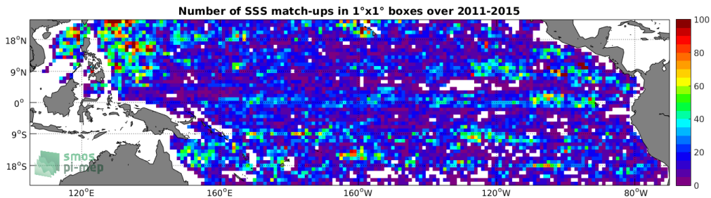
Figure 4: Number of SSS match-ups between Argo SSS and the Aquarius SSS L2-AVERAGED CAP v5 (JPL) SSS product for the Tropical Pacific Ocean Pi-MEP region over 1^\circ \times 1^\circ boxes and for the full satellite product period.
