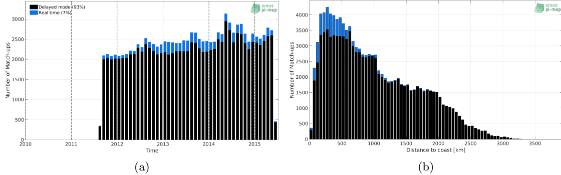
Figure 1: Number of match-ups between Argo and Aquarius SSS L2-AVERAGED CAP v5 (JPL) SSS as a function of time (a) and as function of the distance to coast (b) over the Tropical Pacific Ocean Pi-MEP region and for the full satellite product period.
