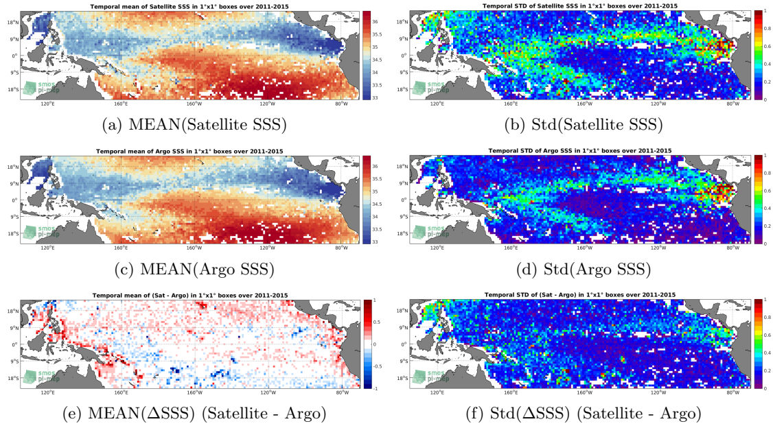
Figure 6: Temporal mean (left) and Std (right) of SSS from Aquarius SSS L2-AVERAGED CAP v5 (JPL) (top), Argo (middle), and of \Delta SSS (Satellite - Argo). Only match-up pairs are used to generate these maps.
