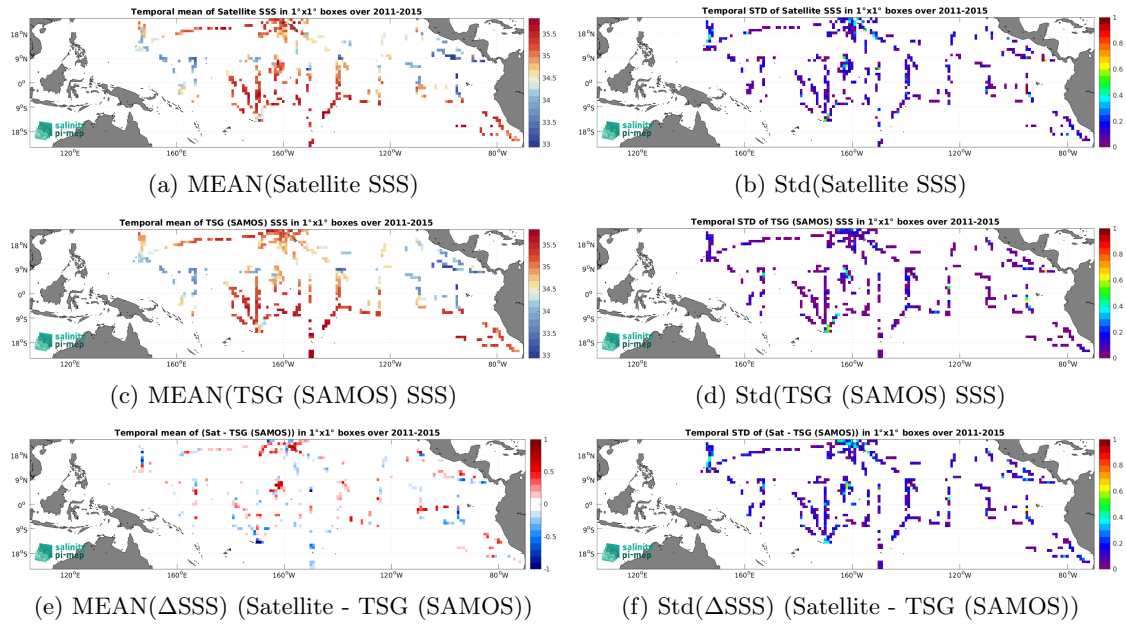
Figure 7: Temporal mean (left) and Std (right) of SSS from Aquarius SSS L2 OR v5 (NASA-GSFC) (top), TSG (SAMOS) (middle), and of \Delta SSS (Satellite - TSG (SAMOS)). Only match-up pairs are used to generate these maps.
