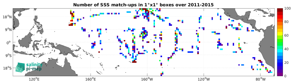
Figure 5: Number of SSS match-ups between TSG (SAMOS) SSS and the Aquarius SSS L2 OR v5 (NASA-GSFC) SSS product for the Tropical Pacific Ocean Pi-MEP region over 1^\circ \times 1^\circ boxes and for the full satellite product period.
