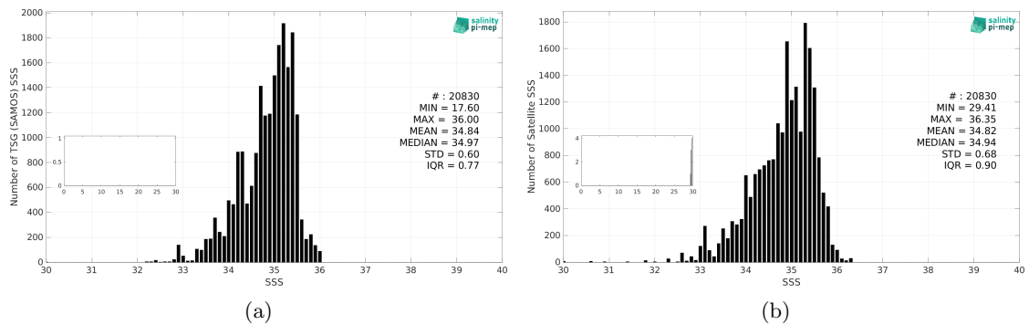
Figure 3: Histograms of SSS from TSG (SAMOS) (a) and Aquarius SSS L2 OR v5 (NASA-GSFC) (b) considering all match-up pairs per bins of 0.1 over the Tropical Pacific Ocean Pi-MEP region and for the full satellite product period.
