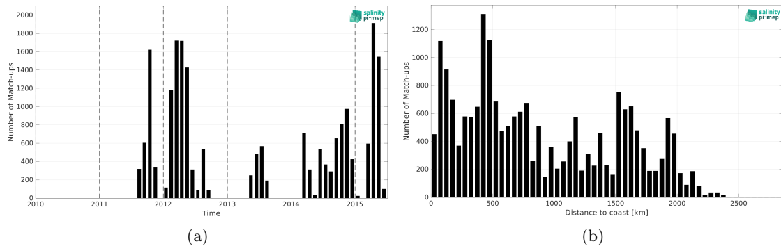
Figure 2: Number of match-ups between TSG (SAMOS) and Aquarius SSS L2 OR v5 (NASA-GSFC) SSS as a function of time (a) and as function of the distance to coast (b) over the Tropical Pacific Ocean Pi-MEP region and for the full satellite product period.
