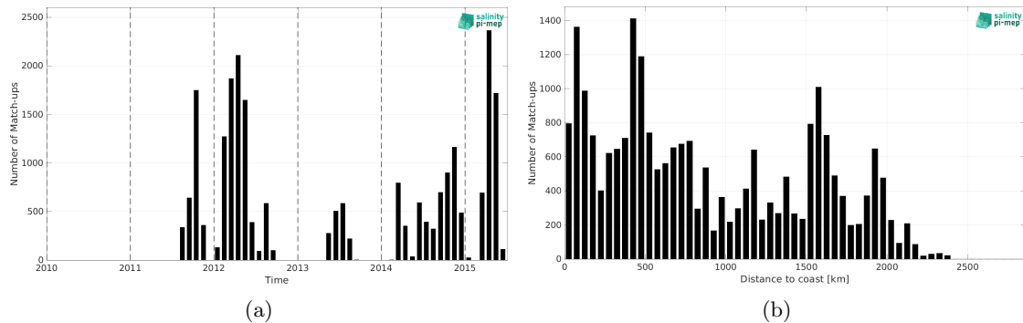
Figure 1: Number of match-ups between TSG (SAMOS) and Aquarius SSS L2 OR v5 (NASA-GSFC) SSS as a function of time (a) and as function of the distance to coast (b) over the Tropical Pacific Ocean Pi-MEP region and for the full satellite product period.
