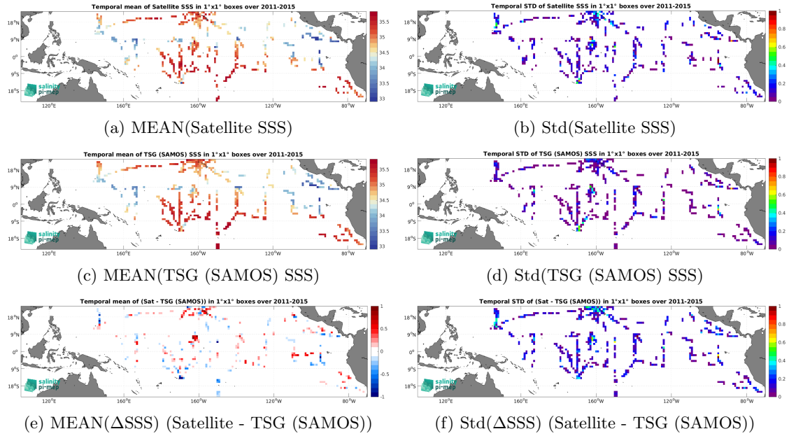
Figure 6: Temporal mean (left) and Std (right) of SSS from Aquarius SSS L2 OR v5 (NASA-GSFC) (top), TSG (SAMOS) (middle), and of \Delta SSS (Satellite - TSG (SAMOS)). Only match-up pairs are used to generate these maps.
