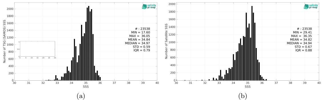
Figure 2: Histograms of SSS from TSG (SAMOS) (a) and Aquarius SSS L2 OR v5 (NASA-GSFC) (b) considering all match-up pairs per bins of 0.1 over the Tropical Pacific Ocean Pi-MEP region and for the full satellite product period.
