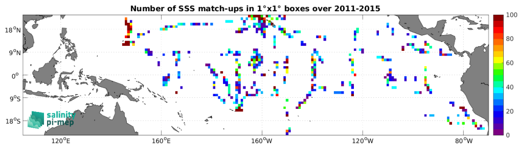
Figure 4: Number of SSS match-ups between TSG (SAMOS) SSS and the Aquarius SSS L2 OR v5 (NASA-GSFC) SSS product for the Tropical Pacific Ocean Pi-MEP region over 1^\circ \times 1^\circ boxes and for the full satellite product period.
