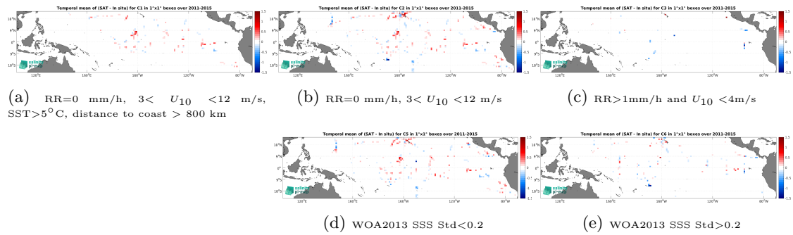
Figure 12: Temporal mean gridded over spatial boxes of size 1^\circ \times 1^\circ of \Delta\text{SSS} (Aquarius SSS L2 OR v5 (NASA-GSFC) - TSG (SAMOS)) for 5 different subdatasets corresponding to: \text{RR}=0 mm/h, 3 < U_{10} < 12 m/s, \text{SST} > 5^\circ\text{C} , distance to coast > 800 km (a), \text{RR}=0 mm/h, 3 < U_{10} < 12 m/s (b), \text{RR} > 1\text{mm/h} and U_{10} < 4\text{m/s} (c), WOA2013 SSS Std < 0.2 (d), WOA2013 SSS Std > 0.2 (e).
