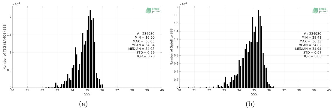
Figure 2: Histograms of SSS from TSG (SAMOS) (a) and Aquarius SSS L2 OR v5 (NASA-GSFC) (b) considering all match-up pairs per bins of 0.1 over the Tropical Pacific Ocean Pi-MEP region and for the full satellite product period.
