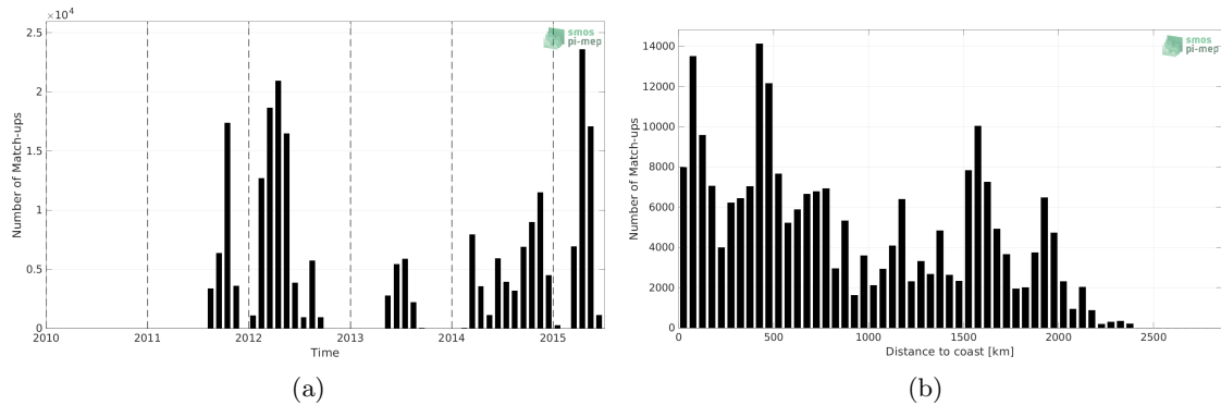
Figure 1: Number of match-ups between TSG (SAMOS) and Aquarius SSS L2 OR v5 (NASA-GSFC) SSS as a function of time (a) and as function of the distance to coast (b) over the Tropical Pacific Ocean Pi-MEP region and for the full satellite product period.
