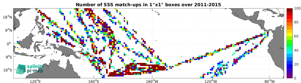
Figure 5: Number of SSS match-ups between TSG (LEGOS-DM) SSS and the Aquarius SSS L2 OR v5 (NASA-GSFC) SSS product for the Tropical Pacific Ocean Pi-MEP region over 1^\circ \times 1^\circ boxes and for the full satellite product period.
