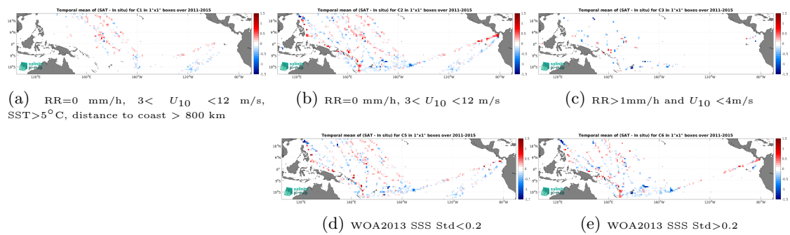
Figure 14: Temporal mean gridded over spatial boxes of size 1^\circ \times 1^\circ of \Delta SSS (Aquarius SSS L2 OR v5 (NASA-GSFC) - TSG (LEGOS-DM)) for 5 different subdatasets corresponding to:RR=0 mm/h, 3 < U_{10} < 12 m/s, SST >5^\circ\text{C} , distance to coast > 800 km (a), RR=0 mm/h, 3 < U_{10} < 12 m/s (b), RR >1 mm/h and U_{10} < 4 m/s (c), WOA2013 SSS Std <0.2 (d), WOA2013 SSS Std >0.2 (e).
