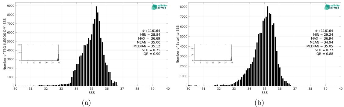
Figure 3: Histograms of SSS from TSG (LEGOS-DM) (a) and Aquarius SSS L2 OR v5 (NASA-GSFC) (b) considering all match-up pairs per bins of 0.1 over the Tropical Pacific Ocean Pi-MEP region and for the full satellite product period.
