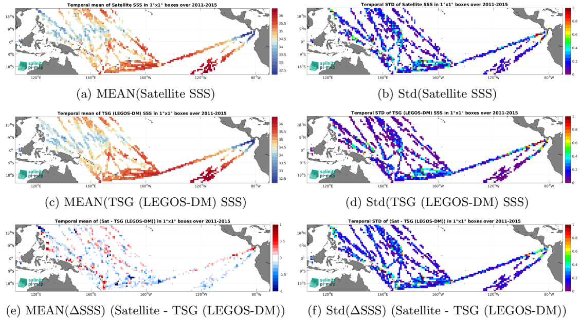
Figure 7: Temporal mean (left) and Std (right) of SSS from Aquarius SSS L2 OR v5 (NASA-GSFC) (top), TSG (LEGOS-DM) (middle), and of \Delta SSS (Satellite - TSG (LEGOS-DM)). Only match-up pairs are used to generate these maps.
