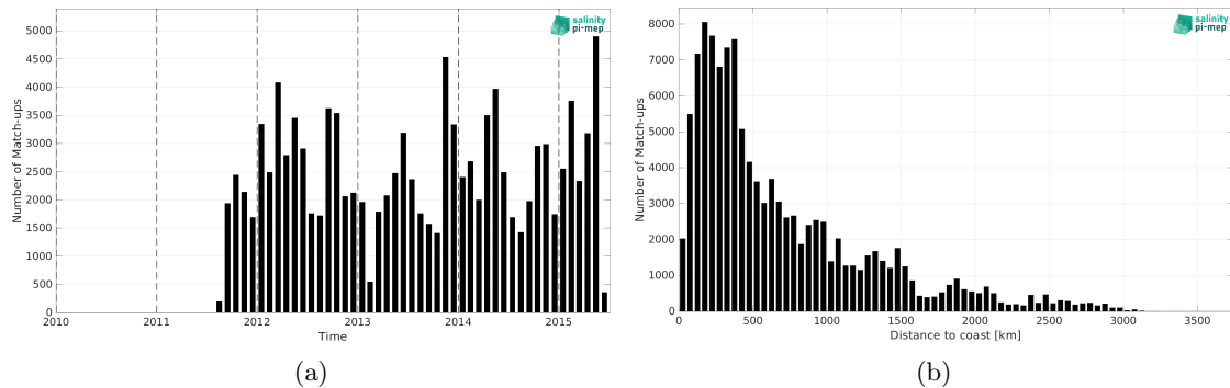
Figure 2: Number of match-ups between TSG (LEGOS-DM) and Aquarius SSS L2 OR v5 (NASA-GSFC) SSS as a function of time (a) and as function of the distance to coast (b) over the Tropical Pacific Ocean Pi-MEP region and for the full satellite product period.
