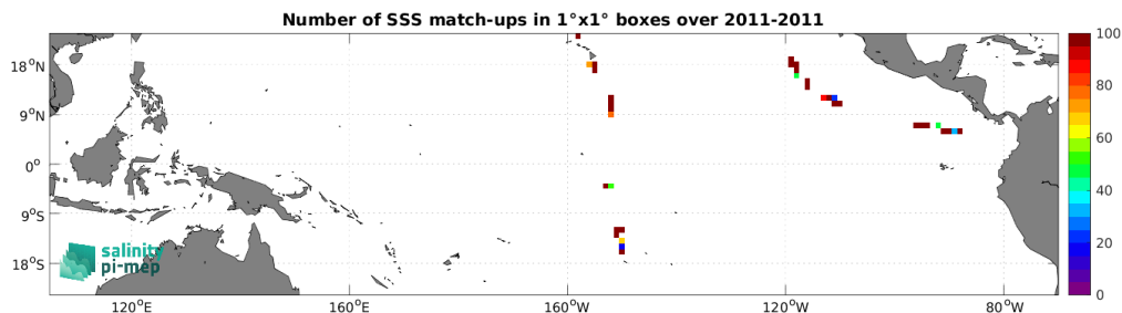
Figure 5: Number of SSS match-ups between TSG (GOSUD-Sailing-ship) SSS and the Aquarius SSS L2 OR v5 (NASA-GSFC) SSS product for the Tropical Pacific Ocean Pi-MEP region over 1^\circ \times 1^\circ boxes and for the full satellite product period.
