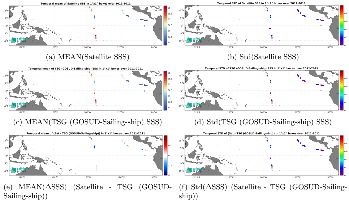
Figure 7: Temporal mean (left) and Std (right) of SSS from Aquarius SSS L2 OR v5 (NASA-GSFC) (top), TSG (GOSUD-Sailing-ship) (middle), and of \Delta SSS (Satellite - TSG (GOSUD-Sailing-ship)). Only match-up pairs are used to generate these maps.
