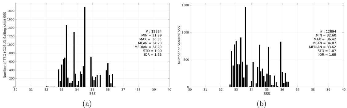
Figure 3: Histograms of SSS from TSG (GOSUD-Sailing-ship) (a) and Aquarius SSS L2 OR v5 (NASA-GSFC) (b) considering all match-up pairs per bins of 0.1 over the Tropical Pacific Ocean Pi-MEP region and for the full satellite product period.
