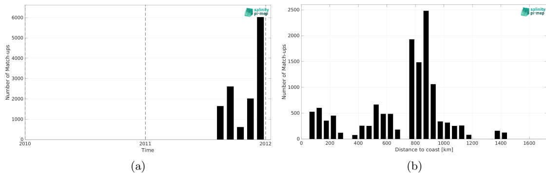
Figure 2: Number of match-ups between TSG (GOSUD-Sailing-ship) and Aquarius SSS L2 OR v5 (NASA-GSFC) SSS as a function of time (a) and as function of the distance to coast (b) over the Tropical Pacific Ocean Pi-MEP region and for the full satellite product period.
