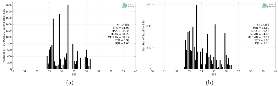
Figure 2: Histograms of SSS from TSG (GOSUD-Sailing-ship) (a) and Aquarius SSS L2 OR v5 (NASA-GSFC) (b) considering all match-up pairs per bins of 0.1 over the Tropical Pacific Ocean Pi-MEP region and for the full satellite product period.
