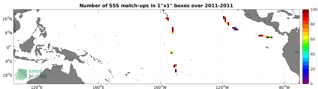
Figure 4: Number of SSS match-ups between TSG (GOSUD-Sailing-ship) SSS and the Aquarius SSS L2 OR v5 (NASA-GSFC) SSS product for the Tropical Pacific Ocean Pi-MEP region over 1^\circ \times 1^\circ boxes and for the full satellite product period.
