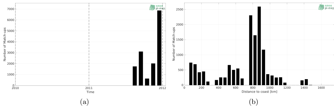
Figure 1: Number of match-ups between TSG (GOSUD-Sailing-ship) and Aquarius SSS L2 OR v5 (NASA-GSFC) SSS as a function of time (a) and as function of the distance to coast (b) over the Tropical Pacific Ocean Pi-MEP region and for the full satellite product period.
