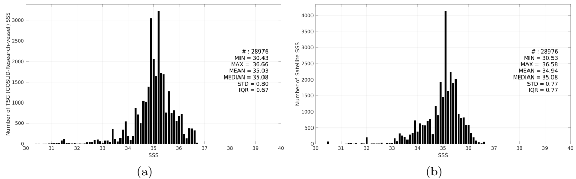
Figure 3: Histograms of SSS from TSG (GOSUD-Research-vessel) (a) and Aquarius SSS L2 OR v5 (NASA-GSFC) (b) considering all match-up pairs per bins of 0.1 over the Tropical Pacific Ocean Pi-MEP region and for the full satellite product period.
