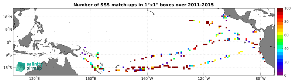
Figure 5: Number of SSS match-ups between TSG (GOSUD-Research-vessel) SSS and the Aquarius SSS L2 OR v5 (NASA-GSFC) SSS product for the Tropical Pacific Ocean Pi-MEP region over 1^\circ \times 1^\circ boxes and for the full satellite product period.
