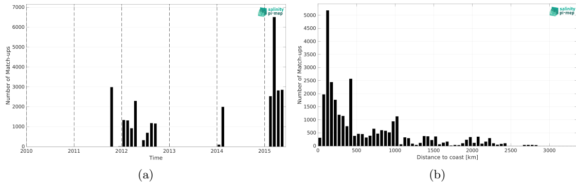
Figure 2: Number of match-ups between TSG (GOSUD-Research-vessel) and Aquarius SSS L2 OR v5 (NASA-GSFC) SSS as a function of time (a) and as function of the distance to coast (b) over the Tropical Pacific Ocean Pi-MEP region and for the full satellite product period.
