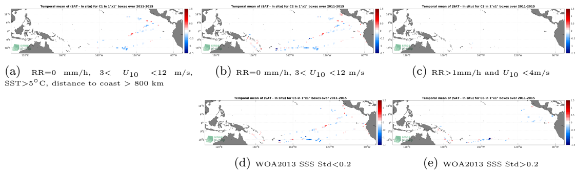
Figure 12: Temporal mean gridded over spatial boxes of size 1^\circ \times 1^\circ of \Delta SSS (Aquarius SSS L2 OR v5 (NASA-GSFC) - TSG (GOSUD-Research-vessel)) for 5 different subdatasets corresponding to: RR=0 mm/h, 3 < U_{10} < 12 m/s, SST > 5°C, distance to coast > 800 km (a), RR=0 mm/h, 3 < U_{10} < 12 m/s (b), RR > 1mm/h and U_{10} < 4 m/s (c), WOA2013 SSS Std < 0.2 (d), WOA2013 SSS Std > 0.2 (e).
