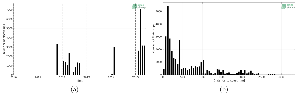
Figure 1: Number of match-ups between TSG (GOSUD-Research-vessel) and Aquarius SSS L2 OR v5 (NASA-GSFC) SSS as a function of time (a) and as function of the distance to coast (b) over the Tropical Pacific Ocean Pi-MEP region and for the full satellite product period.
