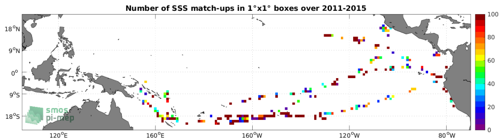
Figure 4: Number of SSS match-ups between TSG (GOSUD-Research-vessel) SSS and the Aquarius SSS L2 OR v5 (NASA-GSFC) SSS product for the Tropical Pacific Ocean Pi-MEP region over 1^\circ \times 1^\circ boxes and for the full satellite product period.
