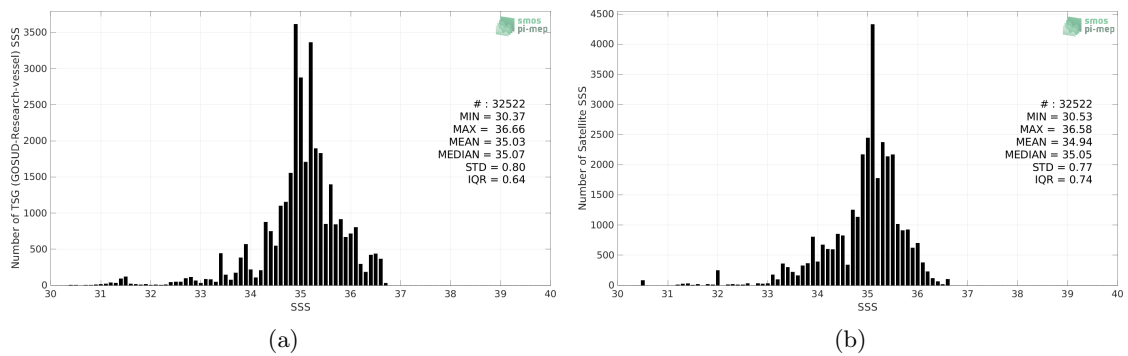
Figure 2: Histograms of SSS from TSG (GOSUD-Research-vessel) (a) and Aquarius SSS L2 OR v5 (NASA-GSFC) (b) considering all match-up pairs per bins of 0.1 over the Tropical Pacific Ocean Pi-MEP region and for the full satellite product period.
