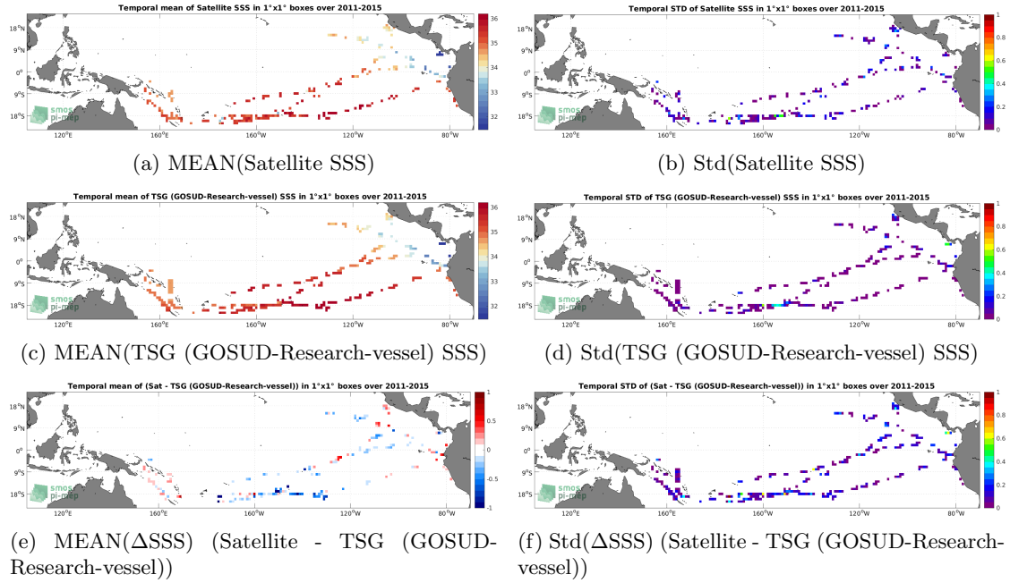
Figure 6: Temporal mean (left) and Std (right) of SSS from Aquarius SSS L2 OR v5 (NASA-GSFC) (top), TSG (GOSUD-Research-vessel) (middle), and of \Delta SSS (Satellite - TSG (GOSUD-Research-vessel)). Only match-up pairs are used to generate these maps.
