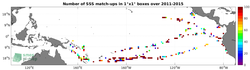
Figure 4: Number of SSS match-ups between TSG (GOSUD-Research-vessel) SSS and the Aquarius SSS L2 OR v5 (NASA-GSFC) SSS product for the Tropical Pacific Ocean Pi-MEP region over 1^\circ \times 1^\circ boxes and for the full satellite product period.
