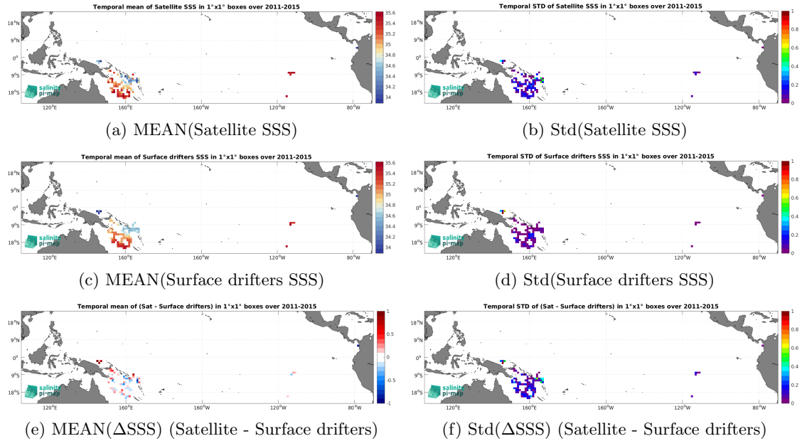
Figure 6: Temporal mean (left) and Std (right) of SSS from Aquarius SSS L2 OR v5 (NASA-GSFC) (top), Surface drifters (middle), and of \Delta SSS (Satellite - Surface drifters). Only match-up pairs are used to generate these maps.
