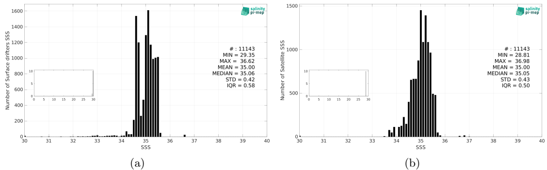
Figure 3: Histograms of SSS from Surface drifters (a) and Aquarius SSS L2 OR v5 (NASA-GSFC) (b) considering all match-up pairs per bins of 0.1 over the Tropical Pacific Ocean Pi-MEP region and for the full satellite product period.
