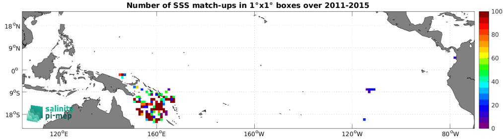
Figure 4: Number of SSS match-ups between Surface drifters SSS and the Aquarius SSS L2 OR v5 (NASA-GSFC) SSS product for the Tropical Pacific Ocean Pi-MEP region over 1^\circ \times 1^\circ boxes and for the full satellite product period.
