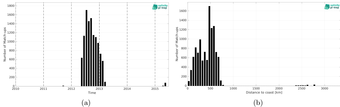
Figure 2: Number of match-ups between Surface drifters and Aquarius SSS L2 OR v5 (NASA-GSFC) SSS as a function of time (a) and as function of the distance to coast (b) over the Tropical Pacific Ocean Pi-MEP region and for the full satellite product period.
