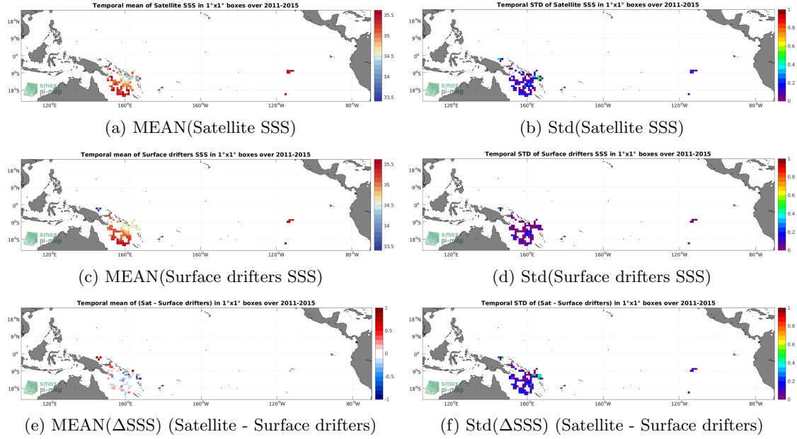
Figure 5: Temporal mean (left) and Std (right) of SSS from Aquarius SSS L2 OR v5 (NASA-GSFC) (top), Surface drifters (middle), and of \Delta\text{SSS} (Satellite - Surface drifters). Only match-up pairs are used to generate these maps.
