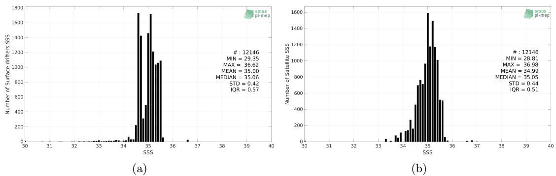
Figure 2: Histograms of SSS from Surface drifters (a) and Aquarius SSS L2 OR v5 (NASA-GSFC) (b) considering all match-up pairs per bins of 0.1 over the Tropical Pacific Ocean Pi-MEP region and for the full satellite product period.
