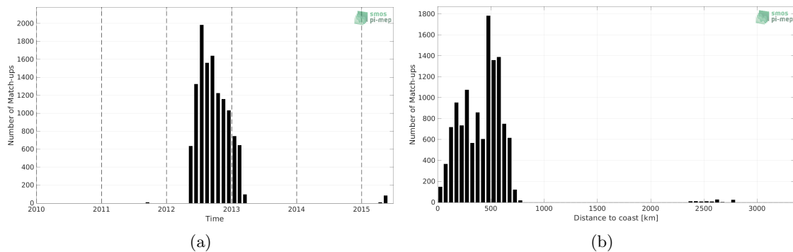
Figure 1: Number of match-ups between Surface drifters and Aquarius SSS L2 OR v5 (NASA-GSFC) SSS as a function of time (a) and as function of the distance to coast (b) over the Tropical Pacific Ocean Pi-MEP region and for the full satellite product period.
