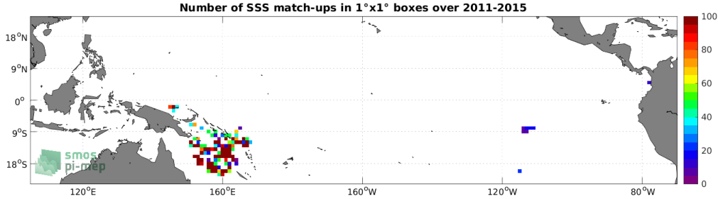
Figure 3: Number of SSS match-ups between Surface drifters SSS and the Aquarius SSS L2 OR v5 (NASA-GSFC) SSS product for the Tropical Pacific Ocean Pi-MEP region over 1^\circ \times 1^\circ boxes and for the full satellite product period.
