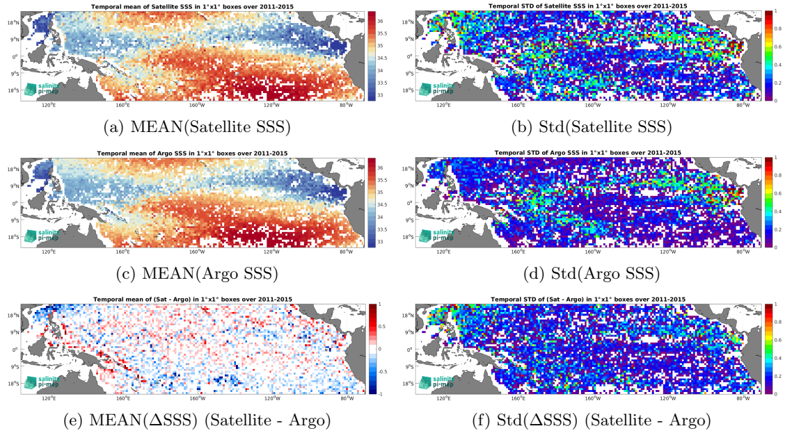
Figure 7: Temporal mean (left) and Std (right) of SSS from Aquarius SSS L2 OR v5 (NASA-GSFC) (top), Argo (middle), and of \Delta SSS (Satellite - Argo). Only match-up pairs are used to generate these maps.
