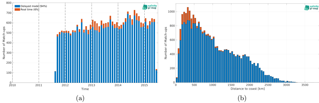
Figure 2: Number of match-ups between Argo and Aquarius SSS L2 OR v5 (NASA-GSFC) SSS as a function of time (a) and as function of the distance to coast (b) over the Tropical Pacific Ocean Pi-MEP region and for the full satellite product period.
