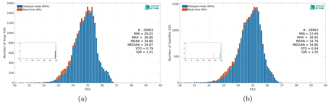
Figure 3: Histograms of SSS from Argo (a) and Aquarius SSS L2 OR v5 (NASA-GSFC) (b) considering all match-up pairs per bins of 0.1 over the Tropical Pacific Ocean Pi-MEP region and for the full satellite product period.
