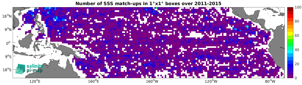
Figure 5: Number of SSS match-ups between Argo SSS and the Aquarius SSS L2 OR v5 (NASA-GSFC) SSS product for the Tropical Pacific Ocean Pi-MEP region over 1^\circ \times 1^\circ boxes and for the full satellite product period.
