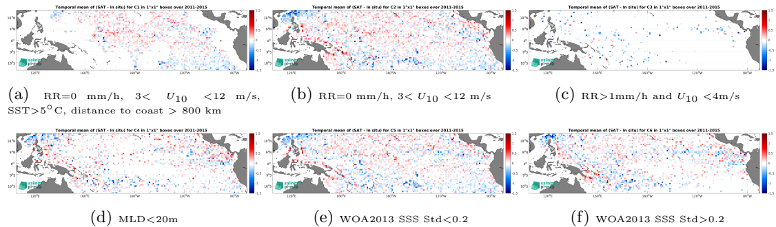
Figure 14: Temporal mean gridded over spatial boxes of size 1^\circ \times 1^\circ of \Delta\text{SSS} (Aquarius SSS L2 OR v5 (NASA-GSFC) - Argo) for 6 different subdatasets corresponding to:RR=0 mm/h, 3 < U_{10} < 12 m/s, SST>5°C, distance to coast > 800 km (a), RR=0 mm/h, 3 < U_{10} < 12 m/s (b), RR>1mm/h and U_{10} < 4 m/s (c),MLD<20m (d),WOA2013 SSS Std<0.2 (e),WOA2013 SSS Std>0.2 (f).
