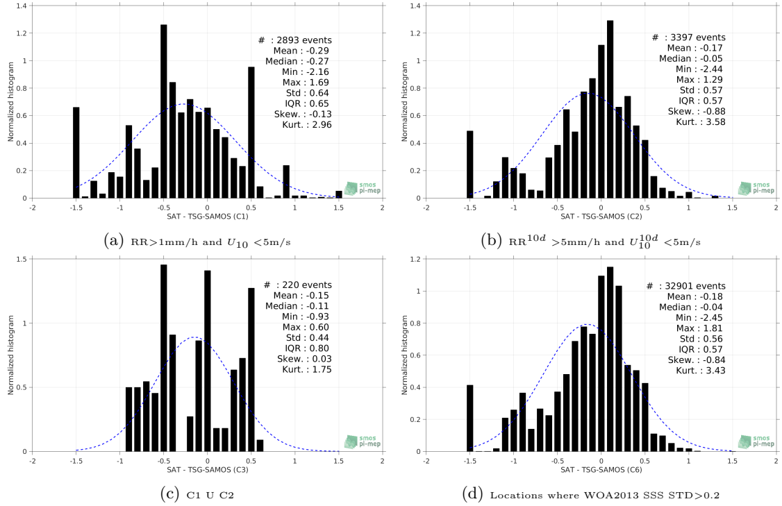
Figure 13: Normalized histogram of \Delta SSS (Aquarius-L2-JPL-V5 - TSG-SAMOS) for 6 different subdatasets corresponding to: RR > 1\text{mm/h} and U_{10} < 5\text{m/s} (a), RR^{10d} > 5\text{mm/h} and U_{10}^{10d} < 5\text{m/s} (b), C1 \cup C2 (c), Locations where WOA2013 SSS STD > 0.2 (d).
