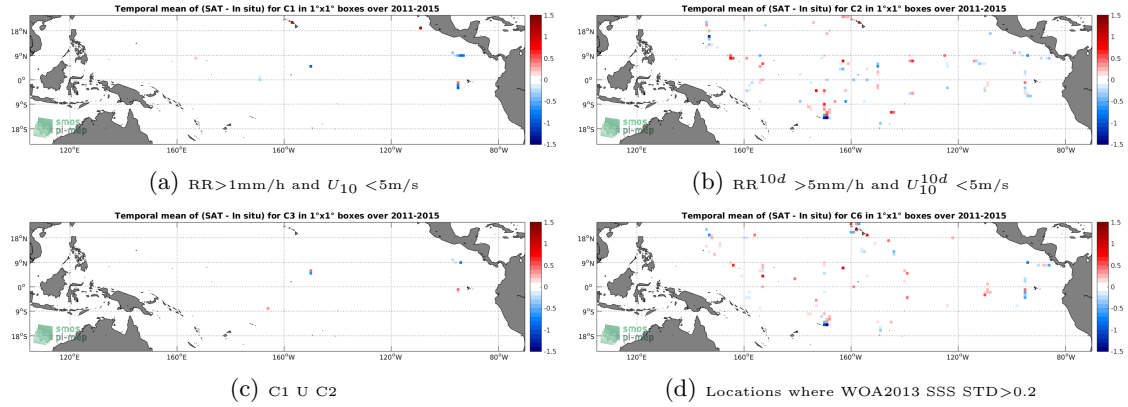
Figure 12: Temporal mean gridded over spatial boxes of size 1^\circ \times 1^\circ of \Delta SSS (Aquarius-L2-JPL-V5 - TSG-SAMOS) for 4 different subdatasets corresponding to: RR > 1\text{mm/h} and U_{10} < 5\text{m/s} (a), RR^{10d} > 5\text{mm/h} and U_{10}^{10d} < 5\text{m/s} (b), C1 U C2 (c), Locations where WOA2013 SSS STD > 0.2 (d).
