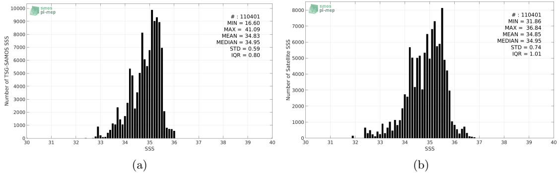
Figure 2: Histograms of SSS from TSG-SAMOS (a) and Aquarius-L2-JPL-V5 (b) considering all match-up pairs per bins of 0.1 over the Tropical Pacific Ocean Pi-MEP region and for the full satellite product period.
