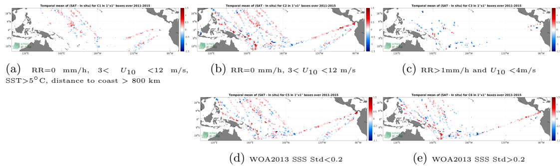
Figure 12: Temporal mean gridded over spatial boxes of size 1^\circ \times 1^\circ of \Delta\text{SSS} (Aquarius SSS L2 CAP v5 (JPL) - TSG (LEGOS-DM)) for 5 different subdatasets corresponding to: RR=0 mm/h, 3 < U_{10} < 12 m/s, SST >5^\circ\text{C} , distance to coast > 800 km (a), RR=0 mm/h, 3 < U_{10} < 12 m/s (b), RR >1 mm/h and U_{10} < 4 m/s (c), WOA2013 SSS Std <0.2 (d), WOA2013 SSS Std >0.2 (e).
