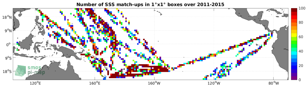
Figure 4: Number of SSS match-ups between TSG (LEGOS-DM) SSS and the Aquarius SSS L2 CAP v5 (JPL) SSS product for the Tropical Pacific Ocean Pi-MEP region over 1^\circ \times 1^\circ boxes and for the full satellite product period.
