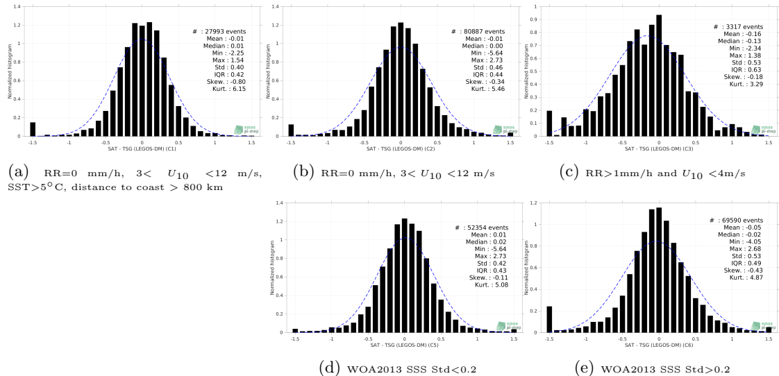
Figure 13: Normalized histogram of \Delta\text{SSS} (Aquarius SSS L2 CAP v5 (JPL) - TSG (LEGOS-DM)) for 5 different subdatasets corresponding to: RR=0 mm/h, 3 < U_{10} < 12 m/s, SST >5^\circ\text{C} , distance to coast > 800 km (a), RR=0 mm/h, 3 < U_{10} < 12 m/s (b), RR >1 mm/h and U_{10} < 4 m/s (c), WOA2013 SSS Std <0.2 (d), WOA2013 SSS Std >0.2 (e).
