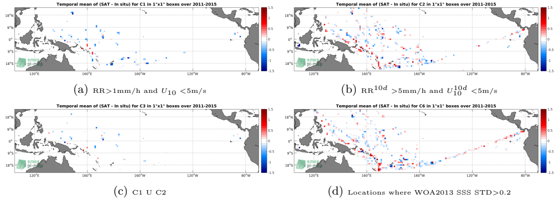
Figure 12: Temporal mean gridded over spatial boxes of size 1^\circ \times 1^\circ of \Delta SSS (Aquarius-L2-JPL-V5 - TSG-LEGOS-DM) for 4 different subdatasets corresponding to: RR > 1mm/h and U_{10} < 5\text{m/s} (a), RR^{10d} > 5\text{mm/h} and U_{10}^{10d} < 5\text{m/s} (b), C1 U C2 (c), Locations where WOA2013 SSS STD > 0.2 (d).
