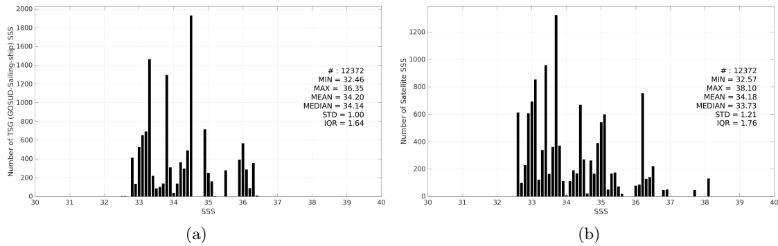
Figure 3: Histograms of SSS from TSG (GOSUD-Sailing-ship) (a) and Aquarius SSS L2 CAP v5 (JPL) (b) considering all match-up pairs per bins of 0.1 over the Tropical Pacific Ocean Pi-MEP region and for the full satellite product period.
