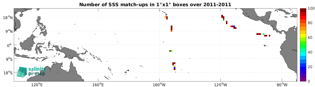
Figure 5: Number of SSS match-ups between TSG (GOSUD-Sailing-ship) SSS and the Aquarius SSS L2 CAP v5 (JPL) SSS product for the Tropical Pacific Ocean Pi-MEP region over 1^\circ \times 1^\circ boxes and for the full satellite product period.
