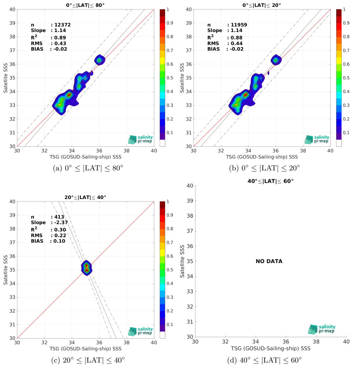
Figure 10: Contour maps of the concentration of Aquarius SSS L2 CAP v5 (JPL) SSS (y-axis) versus TSG (GOSUD-Sailing-ship) SSS (x-axis) at match-up pairs for different latitude bands. For each plot, the red line shows x=y . The black thin and dashed lines indicate a linear fit through the data cloud and the \pm 95\% confidence levels, respectively. The number match-up pairs n , the slope and R^2 coefficient of the linear fit, the root mean square (RMS) and the mean bias between satellite and in situ data are indicated for each latitude band in each plots.
