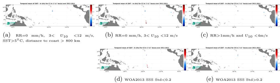
Figure 14: Temporal mean gridded over spatial boxes of size 1^\circ \times 1^\circ of \Delta SSS (Aquarius SSS L2 CAP v5 (JPL) - TSG (GOSUD-Sailing-ship)) for 5 different subdatasets corresponding to: RR=0 mm/h, 3 < U_{10} < 12 m/s, SST > 5^\circ\text{C} , distance to coast > 800 km (a), RR=0 mm/h, 3 < U_{10} < 12 m/s (b), RR > 1 mm/h and U_{10} < 4 m/s (c), WOA2013 SSS Std < 0.2 (d), WOA2013 SSS Std > 0.2 (e).
