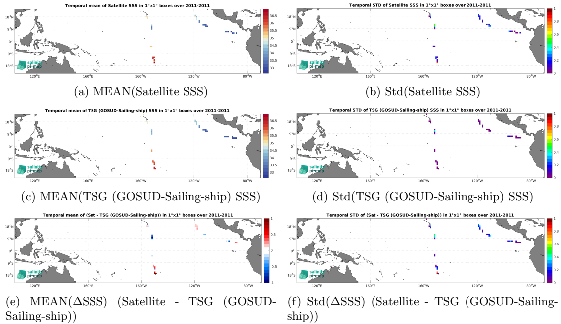
Figure 7: Temporal mean (left) and Std (right) of SSS from Aquarius SSS L2 CAP v5 (JPL) (top), TSG (GOSUD-Sailing-ship) (middle), and of \Delta SSS (Satellite - TSG (GOSUD-Sailing-ship)). Only match-up pairs are used to generate these maps.
