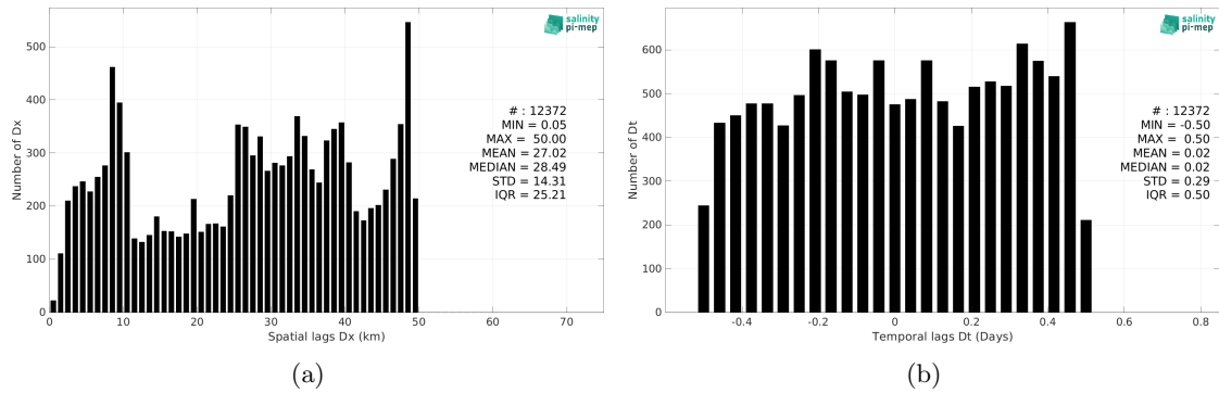
Figure 6: Histograms of the spatial (a) and temporal (b) lags between the location/time of the TSG (GOSUD-Sailing-ship) measurement and the date of the corresponding Aquarius SSS L2 CAP v5 (JPL) SSS pixel.
