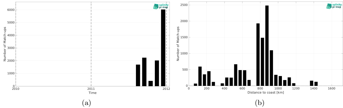
Figure 2: Number of match-ups between TSG (GOSUD-Sailing-ship) and Aquarius SSS L2 CAP v5 (JPL) SSS as a function of time (a) and as function of the distance to coast (b) over the Tropical Pacific Ocean Pi-MEP region and for the full satellite product period.
