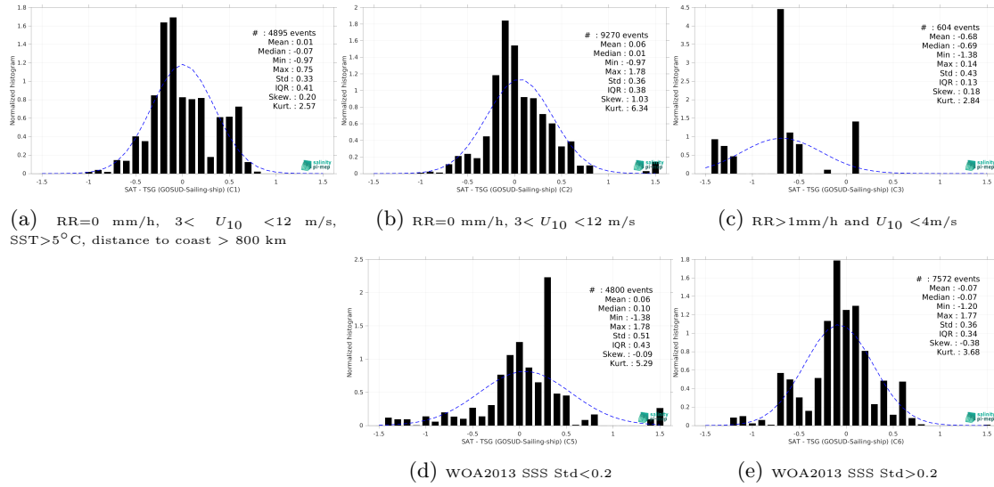
Figure 15: Normalized histogram of \Delta SSS (Aquarius SSS L2 CAP v5 (JPL) - TSG (GOSUD-Sailing-ship)) for 5 different subdatasets corresponding to: RR=0 mm/h, 3 < U_{10} < 12 m/s, SST>5°C, distance to coast > 800 km (a), RR=0 mm/h, 3 < U_{10} < 12 m/s (b), RR>1mm/h and U_{10} < 4 m/s (c), WOA2013 SSS Std<0.2 (d), WOA2013 SSS Std>0.2 (e).
