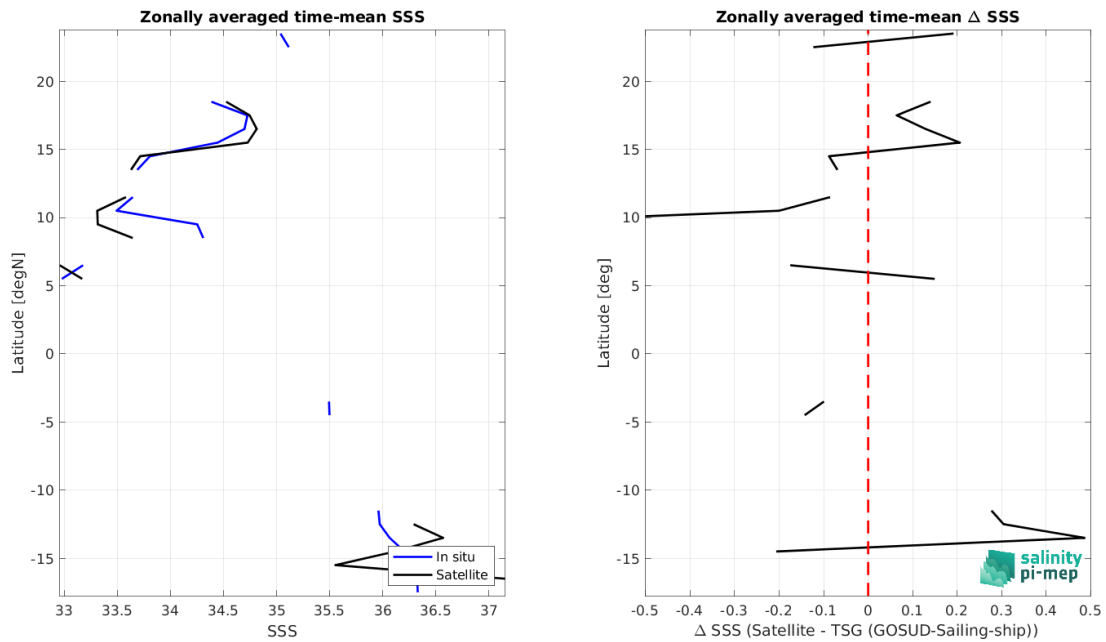
Figure 9: Left panel: Zonal mean SSS from Aquarius SSS L2 CAP v5 (JPL) satellite product (black) and from TSG (GOSUD-Sailing-ship) (blue). Right panel: Zonal mean of \Delta SSS (Satellite - TSG (GOSUD-Sailing-ship)) for all the collected Pi-MEP match-up pairs estimated over the full satellite product period.
