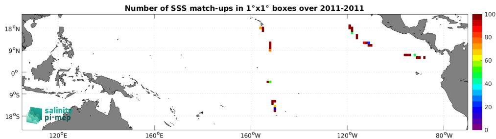
Figure 5: Number of SSS match-ups between TSG (GOSUD-Sailing-ship) SSS and the Aquarius SSS L2 CAP v5 (JPL) SSS product for the Tropical Pacific Ocean Pi-MEP region over 1^\circ \times 1^\circ boxes and for the full satellite product period.
