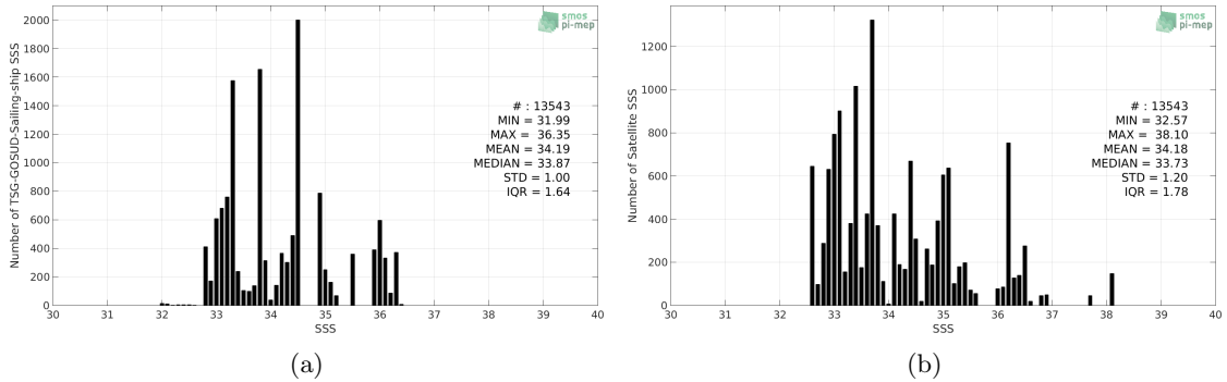
Figure 2: Histograms of SSS from TSG-GOSUD-Sailing-ship (a) and Aquarius-L2-JPL-V5 (b) considering all match-up pairs per bins of 0.1 over the Tropical Pacific Ocean Pi-MEP region and for the full satellite product period.
