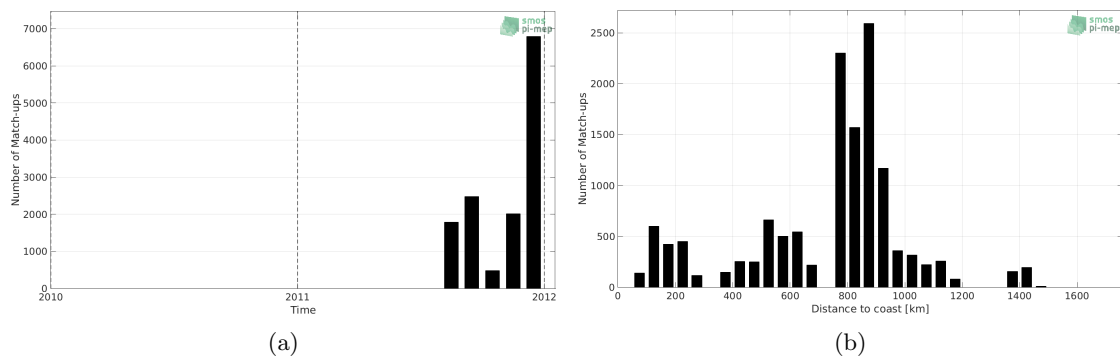
Figure 1: Number of match-ups between TSG-GOSUD-Sailing-ship and Aquarius-L2-JPL-V5 SSS as a function of time (a) and as function of the distance to coast (b) over the Tropical Pacific Ocean Pi-MEP region and for the full satellite product period.
