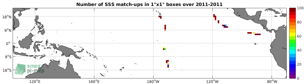
Figure 4: Number of SSS match-ups between TSG-GOSUD-Sailing-ship SSS and the Aquarius-L2-JPL-V5 SSS product for the Tropical Pacific Ocean Pi-MEP region over 1^\circ \times 1^\circ boxes and for the full satellite product period.
