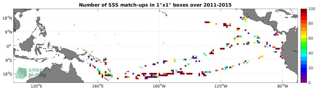
Figure 4: Number of SSS match-ups between TSG (GOSUD-Research-vessel) SSS and the Aquarius SSS L2 CAP v5 (JPL) SSS product for the Tropical Pacific Ocean Pi-MEP region over 1^\circ \times 1^\circ boxes and for the full satellite product period.
