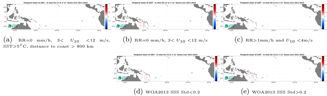
Figure 13: Temporal mean gridded over spatial boxes of size 1^\circ \times 1^\circ of \Delta\text{SSS} (Aquarius SSS L2 CAP v5 (JPL) - Surface drifters) for 5 different subdatasets corresponding to:RR=0 mm/h, 3 < U_{10} < 12 m/s, \text{SST} > 5^\circ\text{C} , distance to coast > 800 km (a), RR=0 mm/h, 3 < U_{10} < 12 m/s (b), RR>1mm/h and U_{10} < 4 m/s (c), WOA2013 SSS Std<0.2 (d), WOA2013 SSS Std>0.2 (e).
