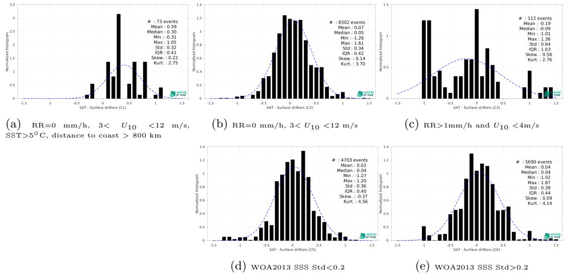
Figure 14: Normalized histogram of \Delta\text{SSS} (Aquarius SSS L2 CAP v5 (JPL) - Surface drifters) for 5 different subdatasets corresponding to: RR=0 mm/h, 3 < U_{10} < 12 m/s, \text{SST} > 5^\circ\text{C} , distance to coast > 800 km (a), RR=0 mm/h, 3 < U_{10} < 12 m/s (b), RR>1mm/h and U_{10} < 4 m/s (c), WOA2013 SSS Std<0.2 (d), WOA2013 SSS Std>0.2 (e).
