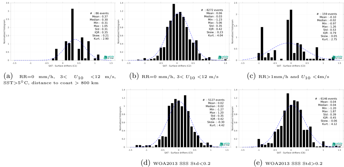
Figure 12: Normalized histogram of \Delta SSS (Aquarius SSS L2 CAP v5 (JPL) - Surface drifters) for 5 different subdatasets corresponding to: RR=0 mm/h, 3 < U_{10} < 12 m/s, SST > 5^\circ\text{C} , distance to coast > 800 km (a), RR=0 mm/h, 3 < U_{10} < 12 m/s (b), RR > 1 mm/h and U_{10} < 4 m/s (c), WOA2013 SSS Std < 0.2 (d), WOA2013 SSS Std > 0.2 (e).
