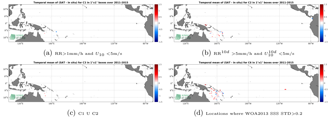
Figure 11: Temporal mean gridded over spatial boxes of size 1^\circ \times 1^\circ of \Delta SSS (Aquarius-L2-JPL-V5 - Surface drifters) for 4 different subdatasets corresponding to: RR > 1mm/h and U_{10} < 5\text{m/s} (a), RR^{10d} > 5\text{mm/h} and U_{10}^{10d} < 5\text{m/s} (b), C1 U C2 (c), Locations where WOA2013 SSS STD > 0.2 (d).
